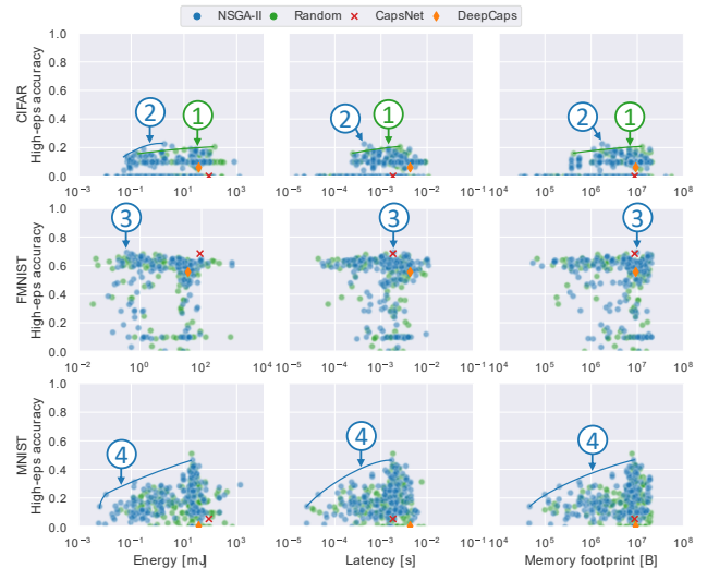
FIGURE 14: RoHNAS ' fast evaluation of DNN robustness under PGD attack in the Two EPS setting using the \epsilon_{high} value, compared to the solutions found with random search, showing tradeoffs w.r.t. energy, latency, and memory footprint.
