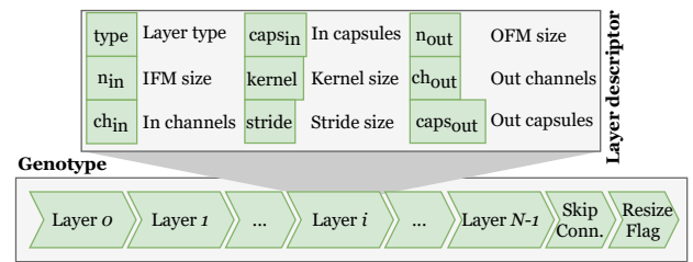
FIGURE 6: Genotype structure. IFM stands for Input Feature Map, while OFM means Output Feature Map.
