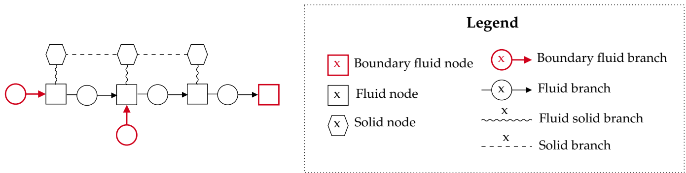
Figure 2. Example of the schematization of a simple system into nodes and branches with indexing practice.
