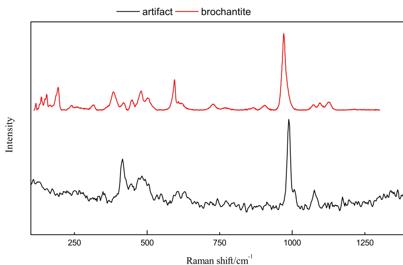
Figure 3. Raman spectrum measured on one bronze figure and reference of brochantite.
