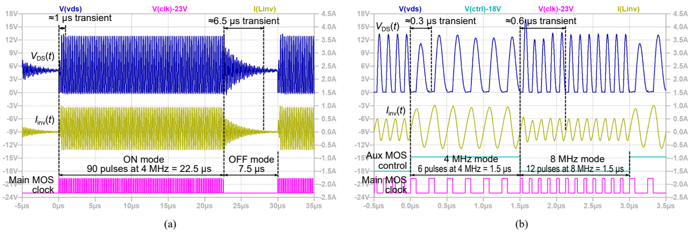
Fig. 4. Drain-to-source voltage V_{DS} and inverter current I_{inv} in a simulation of a controlled class-E boost converter. (a) The time required to turn-off the converter under the ON-OFF control is extremely long, setting the upper bound on the dimming frequency f_d ; (b) transients in the proposed dual-frequency control are extremely short, allowing a much higher f_d .
