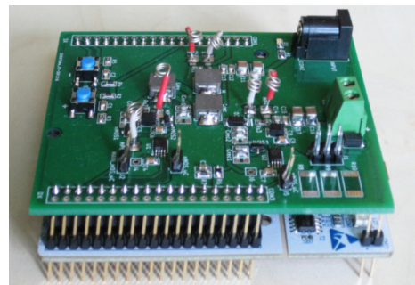
Fig. 7. A picture of the designed prototype that fits on top of the NUCLEO-F334R8 board.
