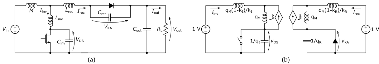
Fig. 2. (a) Basic schematic of the standard class-E boost converter considered in this paper. (b) Schematic of the normalized 1 V – 1 V, 1 W 1 rad/s equivalent class-E converter considered in [15] for the design of the converter in Figure 2(a).
