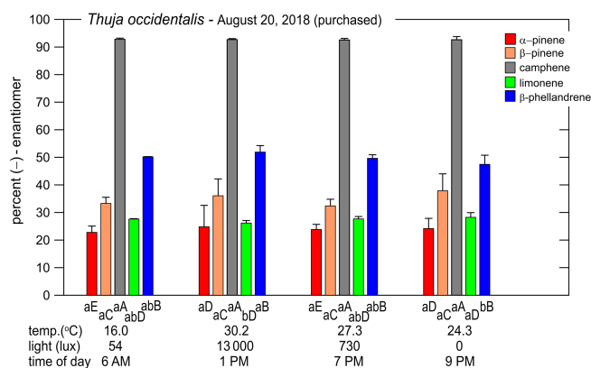
Figure 4. Percent of the (–)-enantiomer for five monoterpenes in nursery-purchased samples of Thuja occidentalis on 20 August 2018. For a given time, the largest value is designated “A”; thereafter, a different capital letter indicates a significant difference between the monoterpenes. For a given monoterpene, the largest value is designated “a”; thereafter, a different lowercase letter indicates a significant difference between the times. The error bars are \pm 1 SD. The data values are given in Table 4.
