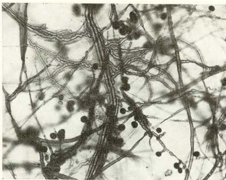
Fig. 5 — Fourteen day culture of Nigrospora sphaerica (Sample 278) on a cellophane disc overlaying Sabouraud's agar. Four month old preparation. No staining, 160 X.
