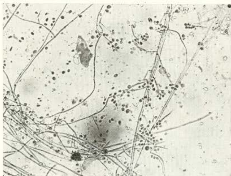
Fig. 3 — Sixteen day culture of Sporotrichum schenckii (Sample 424, Patient MFG., 1972), on a cellophane disc overlaying Fava Netto's medium. Sixteen day old preparation. Amman's lactophenol staining, 400 X.
