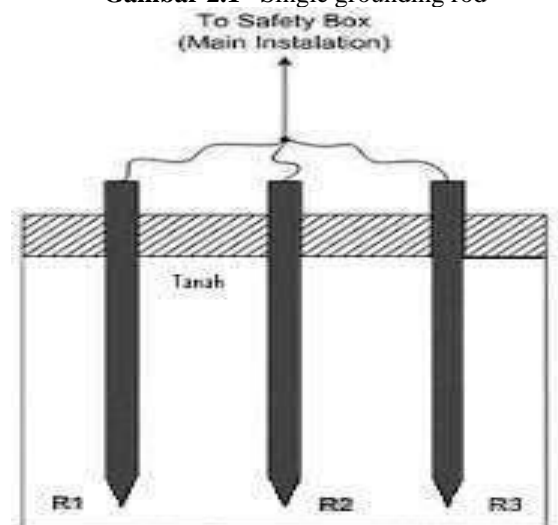
Gambar 2.2 Multiple grounding rod
