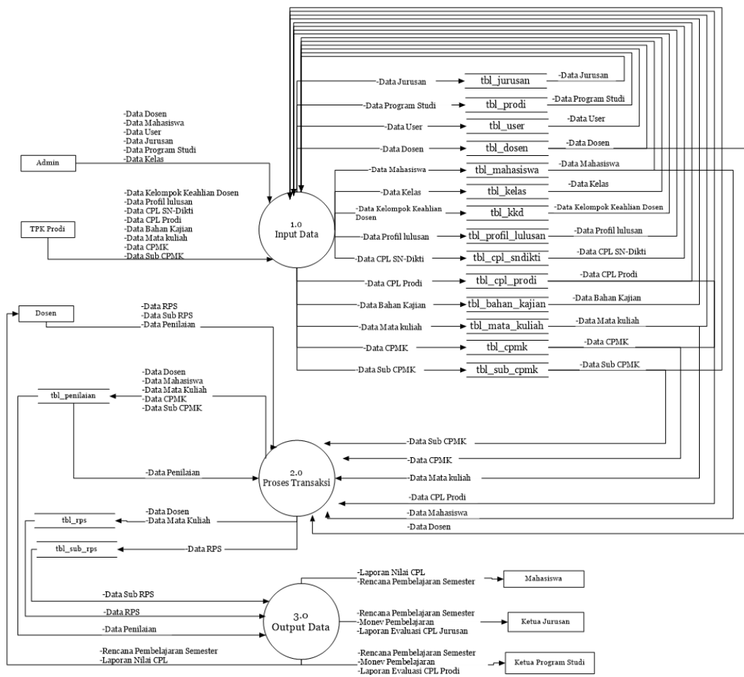
Gambar 2. Diagram Alir Data Level 0
