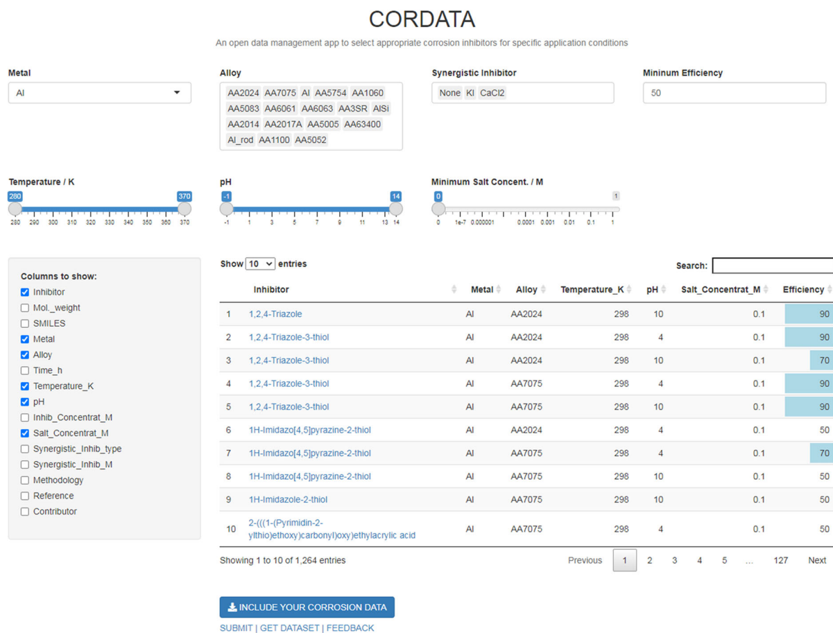
Fig. 1 Graphical user interface (GUI) of the CORDATA web application. The CORDATA GUI ( https://datacor.shinyapps.io/cordata/ ) includes digital features to search and select the data, according to intended application conditions of the corrosion inhibitors, as well as the main table with corrosion inhibition efficiencies and corresponding measurement properties.
