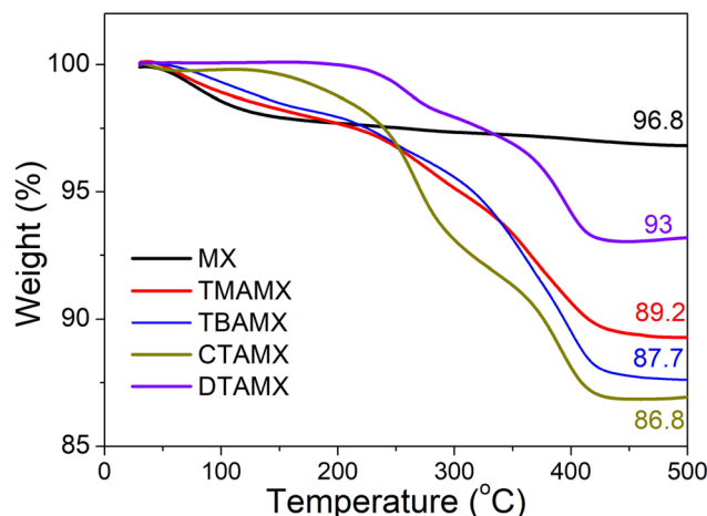
Fig. 1 Thermogravimetric curves of MX, TMAMX, TBAMX, DTAMX and CTAMX in nitrogen at a heating rate of 10\ ^\circ C\ min^{-1} .
