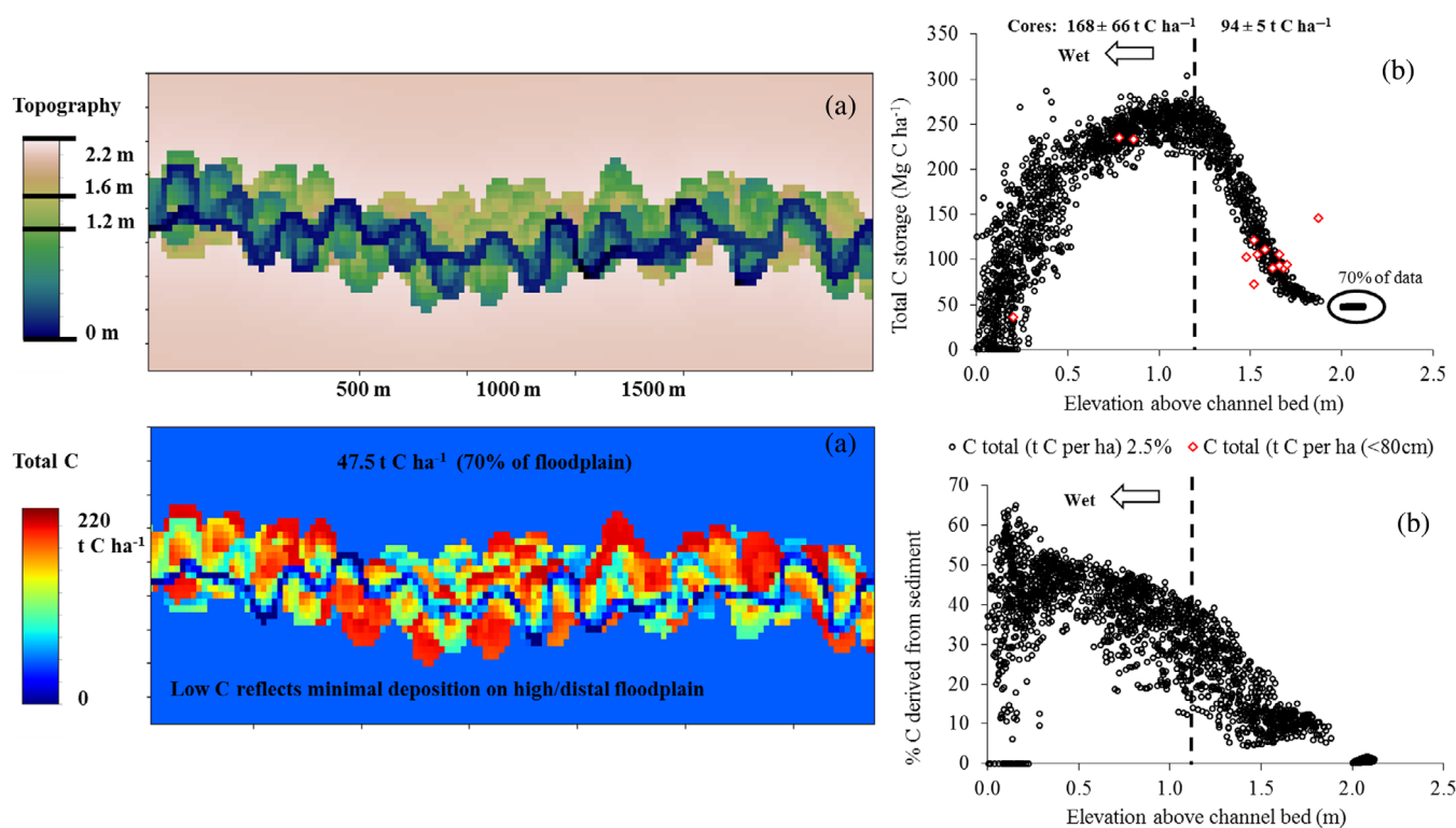
FIGURE 6 Floodplain evolution model demonstrating lowland floodplain topography and associated carbon storage (a); modelled carbon storage and % carbon derived from U_{in} (b), utilizing the elevation of 1.2 m above the channel bed as the boundary between RothC decay rates and the rate perturbed 4-fold slower decomposition in the high deposition ACB, with observed field data of carbon stock over 0.8 m (ACB: n = 3 , floodplain: n = 11 ; panel b).
