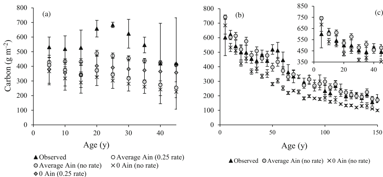
FIGURE 5 Measured carbon content averaged across 5 y intervals for the ACBs (a; n = 3 ) and floodplain (b; n = 11 ) cores on the river culm, with the age profile estimated from the ^{137}\text{Cs} assay or from cut-off formation. ACB cores reached the bedload at approx. 45 y compared to >150 y for floodplain cores. With panels (a) and (b) showing the observed carbon to the modelled carbon and the inset panel (c) the floodplain carbon content over 45 y. Modelled carbon utilized RothC decay coefficients applied to estimates of U_{in} and A_{in} , with average vegetation input of 3.24 \text{ t C ha}^{-1} \text{ y}^{-1} and sediment only ( 0 A_{in} ) model outputs shown. Panel (a) shows the modelled carbon in ACB cores using RothC decay coefficients with the rate adjustment factor (0.25 rate) and without rate adjustment (no rate)
