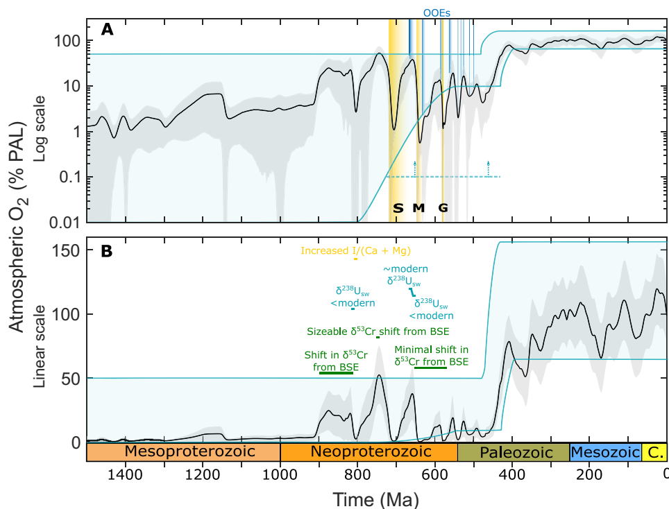
Fig. 3. Reconstructed O_2 evolution from 1500 Ma to present. Atmospheric oxygen results estimated from the NEOCARBSULF model in log (A) and linear (B) forms. In each panel, the black line is the mean result of 5000 model runs, and the gray shaded band represents \pm 1 SD, which may include very low values on occasion. The blue shaded band is the O_2 best guess estimate from Fig. 1A (top panel). In (A), the blue lines are the OOEes as seen in Fig. 1B (bottom panel). The blue dashed line with arrows is the minimum O_2 level previously defined by substantial \delta^{53}\text{Cr} fractionation (23, 24). The yellow lines are the glaciations: S, Sturtian; M, Marinoan; G, Gaskiers. In (B), notable geochemical proxies—see text for further details.
