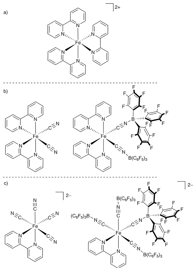
Figure 1. Chemical structures of [\text{Fe}(\text{bpy})_3]^{2+} (a), [\text{Fe}(\text{bpy})_2(\text{CN})_2] and [\text{Fe}(\text{bpy})_2(\text{BCF})_2] (b), and [\text{Fe}(\text{bpy})(\text{CN})_4]^{2-} and [\text{Fe}(\text{bpy})(\text{BCF})_4]^{2-} (c) (BCF = \text{CNB}(\text{C}_6\text{F}_5)_3 ; bpy = 2,2'-bipyridine).
