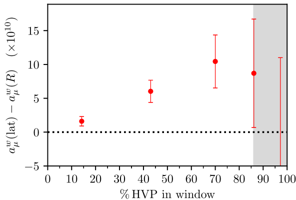
FIG. 10. Difference between determinations of a_\mu^w from the lattice and from R_{e^+e^-} with one-sided windows for a_\mu^w (from left to right) t_1 = 0.5, 1, 1.5, 2 and 3 fm. The differences are plotted versus the fraction of the total HVP included in the window. We have insufficient statistics to give reliable results for t_1 > 2 fm (gray shading).
