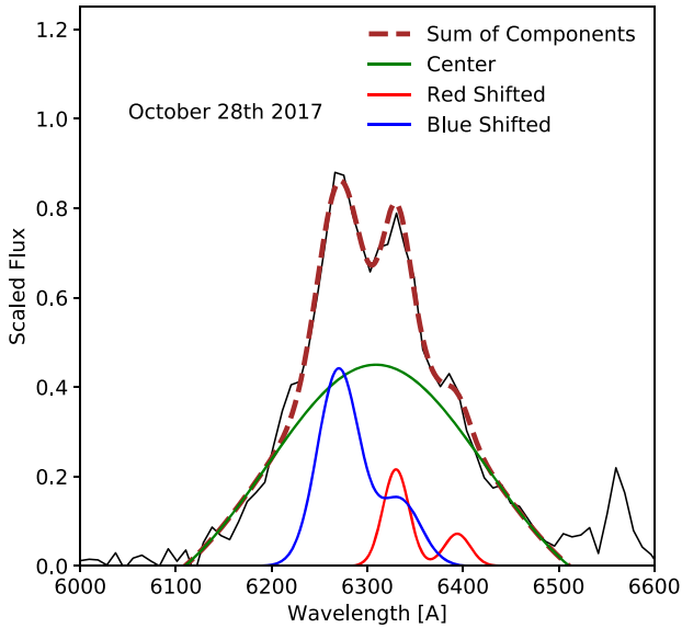
Figure 9. Fits to the [O I] \lambda\lambda 6300, 6363 doublet for the 2017 October 28 spectrum of SN 2017ein using the same method as in Taubenberger et al. (2009). The region around the doublet is normalized and scaled before the fit is applied.
