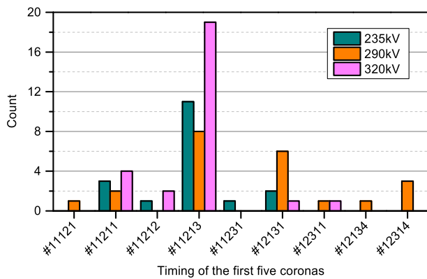
FIGURE 6 Patterns of discharge sequence for the first five corona bursts. Take #1121 for example, it is the abbreviation of #1-#1-#1-#2-#1. Discharge #1 can refer specifically to that at the electrode tip, while #2 and subsequent numbered discharges refer generally to those occurring around the electrode side and do not correspond to a specific location
