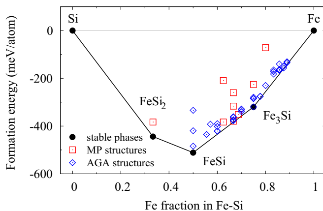
FIG. 3. Phase diagram of a binary Fe-Si system. The formation energies are plotted as a function of the Fe content. Crystal structures are taken from Materials Project (MP) and discovered through our adaptive genetic algorithm (AGA). A set of the solid lines that connect stable phases, called the convex hull, represents the theoretical lower limit in this compositional phase diagram. The closer it is to the convex hull, the more likely it is for the material to exist.
