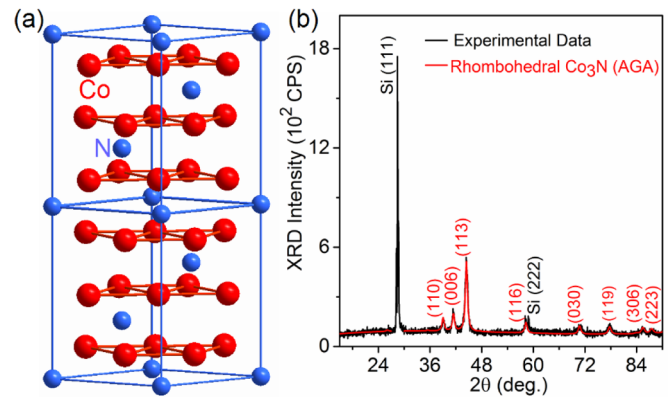
FIG. 11. (a) Schematic of a rhombohedral crystal structure of a Co 3 N compound predicted by the AGA search [31]. (b) The experimental x-ray diffraction (XRD) pattern of the cluster-deposited Co 3 N nanoparticles on a Si (111) substrate (black curve) is fit with the predicted rhombohedral structure using Rietveld analysis (red curve) [32].
