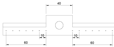
(a) Weight holder diagram (diagram in mm)
