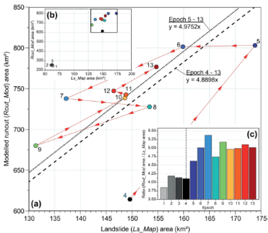
Figure 3. (a) Correlation between per-epoch landslide (Ls_Map) area and modelled runout (Rout_Mod) area. Separate trend lines fitted for (1) epochs 4-13, dashed, and (2) epochs 5-13, dotted, with regression lines both forced through the origin. The red line connects the epochs sequentially by date to indicate changes through time. Panel (b) shows the same data but including the three pre-earthquake epochs 1-3. (c) Ratio of modelled runout (Rout_Mod) area to landslide (Ls_Map) area through time. Higher values indicate greater runout extent relative to the landslide sources. Vertical black dashed line indicates the time of the earthquake (epoch 4).
