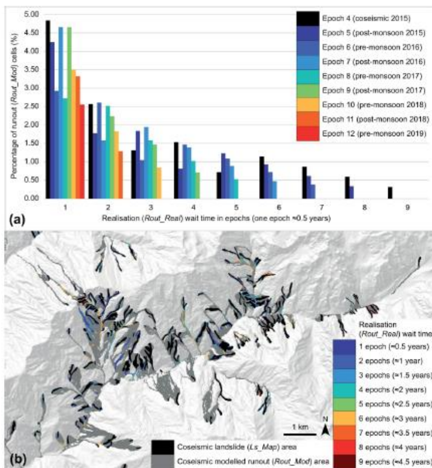
Figure 6. (a) Distribution of runout realisation wait times for all co- and post-seismic epochs. Realisation wait times are defined here as the time between when a cell is first included within a modelled runout area for a given epoch ( Rout\_Mod ), and when it first intersected a mapped landslide polygon ( Rout\_Real ). Note that longer wait times can only be determined for the earlier epochs due to the brevity of our inventory data. (b) Map showing an example of per-cell realisation wait times associated with the modelled coseismic runout for an area of Dolakha district. The spatial extent of this map is shown on Fig. 1 for reference.
