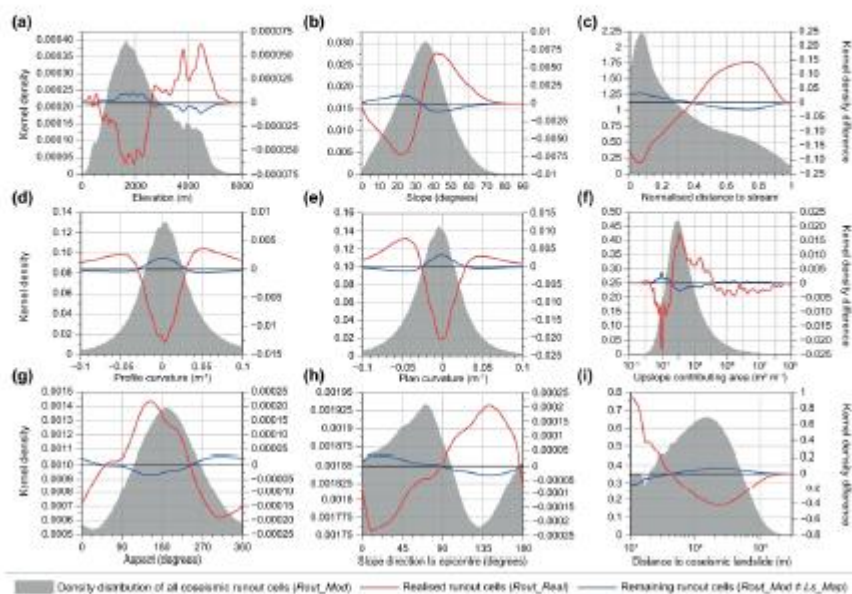
Figure 10. Kernel density distributions of all modelled coseismic runout cells (Rout_Mod) for selected topographic, seismic and distance-based variables. Differences in kernel density values relative to the overall distribution are shown for those cells where the coseismic runout hazard was later realised (Rout_Real; red) and for those where it was not (Rout_Mod \neq Ls_Map; blue). Shaded areas show distributions of each variable for all coseismic runout cells (Rout_Mod) within the study area for reference.
