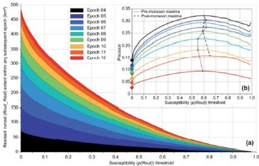
Figure 7. (a) Extent of modelled runout in each of the mapping epochs that was realised by landslide occurrence within any subsequent epoch (Rout_Real), differentiated by susceptibility ( p(\text{Rout}) ) threshold. Note: the realisation area data on the y-axis are stacked. (b) Model precision by epoch, defined as the realised runout area (Rout_Real) as a fraction of the total coseismic runout area (Rout_Mod), again differentiated by susceptibility ( p(\text{Rout}) ) threshold. For all epochs, the model achieves maximum precision at a p(\text{Rout}) threshold of 0.55–0.65; these points are connected for reference to show their evolution in time for both pre- and post-monsoon inventories. Coloured dots on the y-axis indicate the proportion of all Rout_Mod that was realised by the end of the study for each mapping epoch.
