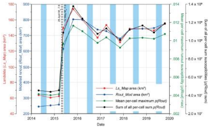
Figure 2. Time series of total landslide area (Ls_Map), runout area (Rout_Mod), and runout susceptibilities ( p(\text{Rout}) ) for the overall study area. Vertical blue bars show the timing of the monsoon; dashed vertical black lines indicate the dates of the 25 April Mw 7.8 Gorkha earthquake and the 12 May Mw 7.3 aftershock. Modified from Kinney et al. (2021) and Rosser et al. (2021).
