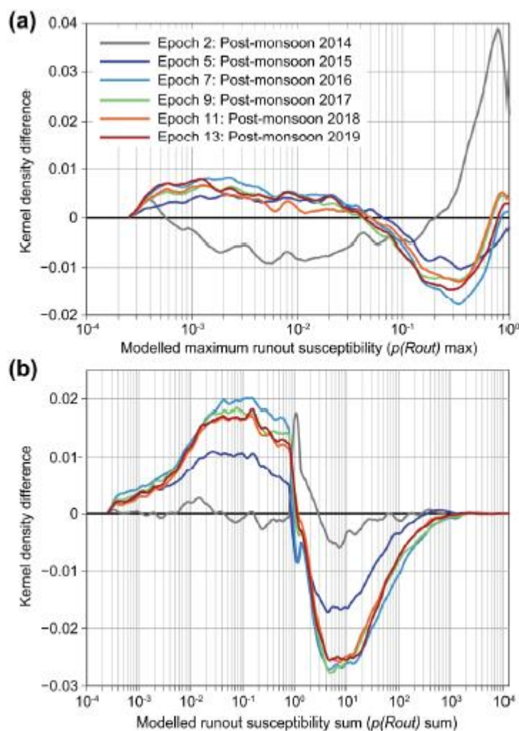
Figure 4. Kernel density estimates of the distributions of (a) maximum per-cell runout susceptibility ( p(Rout) max) and (b) the per-cell sum of all runout susceptibilities ( p(Rout) sum), expressed as the difference between each distribution and the coseismic distribution in epoch 4 (black line). Positive values represent a greater number of cells with corresponding value of p(Rout) , negative value represent a smaller number of cells relative to epoch 4.
