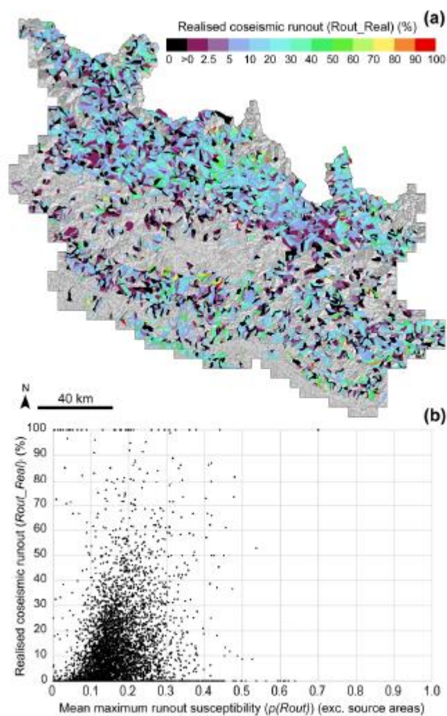
Figure 9. (a) Realised coseismic runout (Rout_Real) plotted by individual slope unit. Values indicate the percentage of cells in each slope unit that were modelled as part of the coseismic runout area (Rout_Mod), and were then occupied by a landslide in any post-seismic epoch (Ls_Map). (b) Scatter plot of per-slope unit realised coseismic runout (Rout_Real) (%) against the mean of all maximum runout susceptibility ( p(Rout) ) values within each corresponding slope unit. Note: data are only plotted for slope units that include runout cells.
