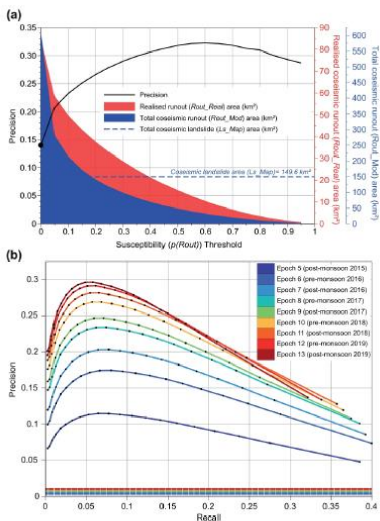
Figure 5. (a) Area of modelled coseismic runout ( Rout\_Mod ; blue) and area of modelled coseismic runout that was realised by landslide occurrence within any post-EQ epoch ( Rout\_Real ; red), as a function of modelled susceptibility p(Rout) threshold. The black line shows the model precision, defined as the realised runout area ( Rout\_Real ) as a fraction of the total coseismic runout area ( Rout\_Mod ), again as a function of susceptibility ( p(Rout) ) threshold. The maximum model precision occurs at a p(Rout) threshold of 0.6. Black dot on the y-axis indicates that 14% of all coseismic Rout\_Mod was realised by the end of the study. (b) Precision-recall curves for each of the post-seismic epochs, based on modelling of runout from coseismic (epoch 4) landslides and comparison with subsequent mapped landslide inventories (epochs 5-13). Each curve is calculated based on the cumulative extent of post-seismic landsliding that occurred up until that epoch. Black dots along the curve represent the susceptibility thresholds, increasing in 0.05 intervals from zero. Horizontal dashed lines towards the base of the y-axis show the no skill values for a random classifier from each epoch; note that the precision depends upon the number of positive values, and so varies between epochs.
