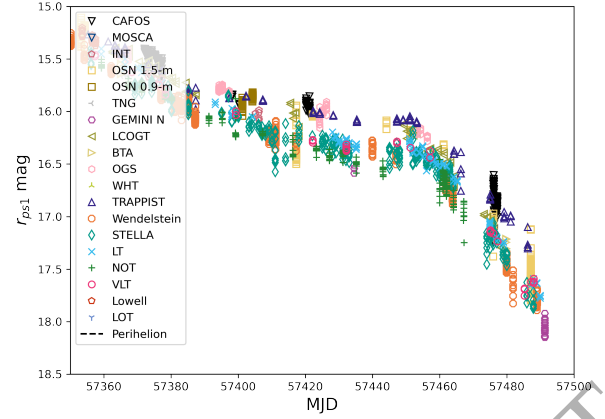
Figure 3. Light curve around low phase angles. All points have been calibrated to r PS1 band. A clear offset is seen in the TRAPPIST (blue triangles), OSN (yellow squares), OGS (pink hexagons) and CAFOS (black downward-triangles) points which were measured in Johnson/Cousin R filter. The majority of the other points were measured in Sloan- r type filters.
