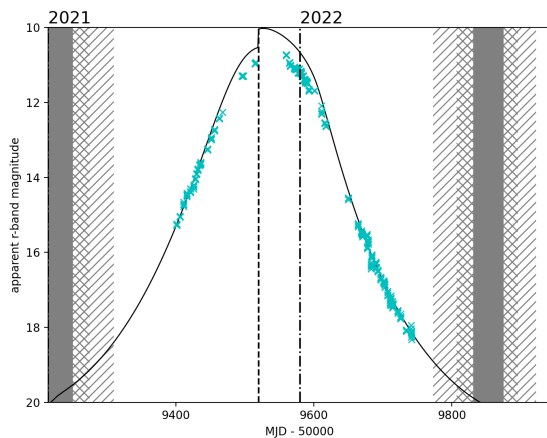
Figure 8. r -band light curve of the 2021–2022 67P apparition. Observations were taken at the LT. The solid black curve is the predicted brightness of the comet. The step in the curve between pre- and post-perihelion is not a real feature and is due to the simplistic power law functions used in the prediction. The vertical dashed line shows the time of perihelion. The hatched patterns shows when solar elongation below 50^\circ (hatched), 30^\circ (cross-hatched) and 15^\circ (solid grey). The dash-dotted line shows the division between years. The photometry behind this plot can be found in Table A3.
