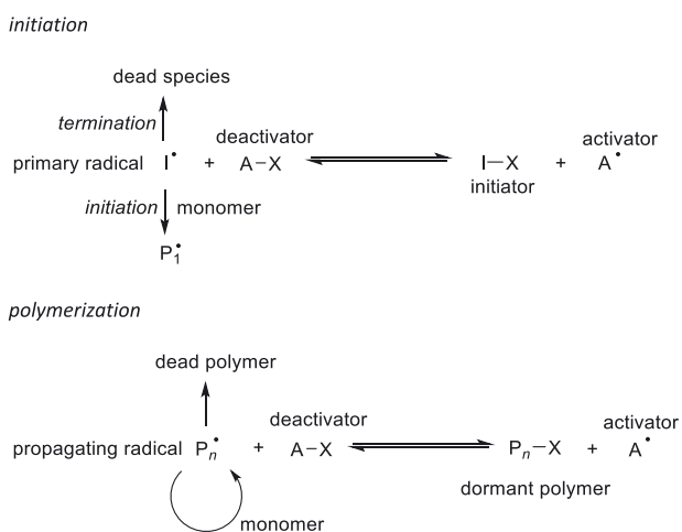
Scheme 5: Non-metal-mediated atom-transfer radical polymerization (NM-ATRP). I^{\bullet} is a primary radical. P_n^{\bullet} is an active species, a propagating radical of chain length n . A-X is a deactivator. A^{\bullet} is an activator.
