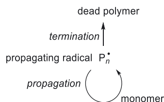
Scheme 1: Simplified mechanism for radical polymerization . I^\bullet is a primary radical . P_n^\bullet is an active species , a propagating radical of chain length n , and contains the active centre .
