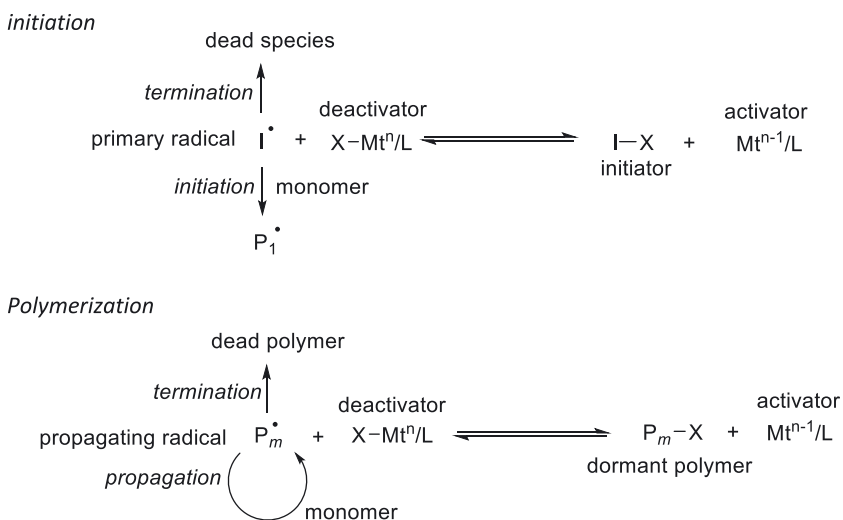
Scheme 4: Transition metal-mediated atom-transfer radical polymerization (TM-ATRP or ATRP). I^{\bullet} is a primary radical. P_m^{\bullet} is an active species, a propagating radical of chain length m . X-Mt^n/L is a deactivator ( Mt^n is transition metal in a higher oxidation state, L is a ligand). Mt^{n-1}/L is an activator ( Mt^{n-1} is a transition metal in a lower oxidation state).
