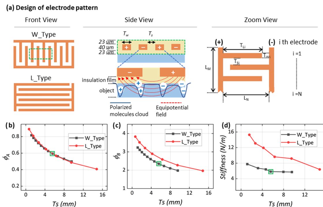
Figure 5. Design of the electrode pattern for the bio-based metasurface. The design is based on the adhesive force and the bending stiffness. (a) Electrode pattern is designed for different configurations (W_type or L_type), electrode lengths, and widths T_L and T_w , and the space between two electrodes T_s . Equipotential field distributions generated by the two in-plane electrodes propagating in the out-of-plane direction provide the maximum charges accumulated in the areas of the object corresponding to the boundary edges of the electrodes so that higher \phi_A and \phi_B fractions help to achieve larger adhesive forces; their relationship with T_s is shown in panels (b) and (c). Lower bending stiffness provides less resistance when the bio-based HyTemC is actuated. (d) W_type configuration and wider space between electrodes help to lower the bending stiffness. The selected type of electrode positioning and T_s value for the final design are indicated by the green squares.
