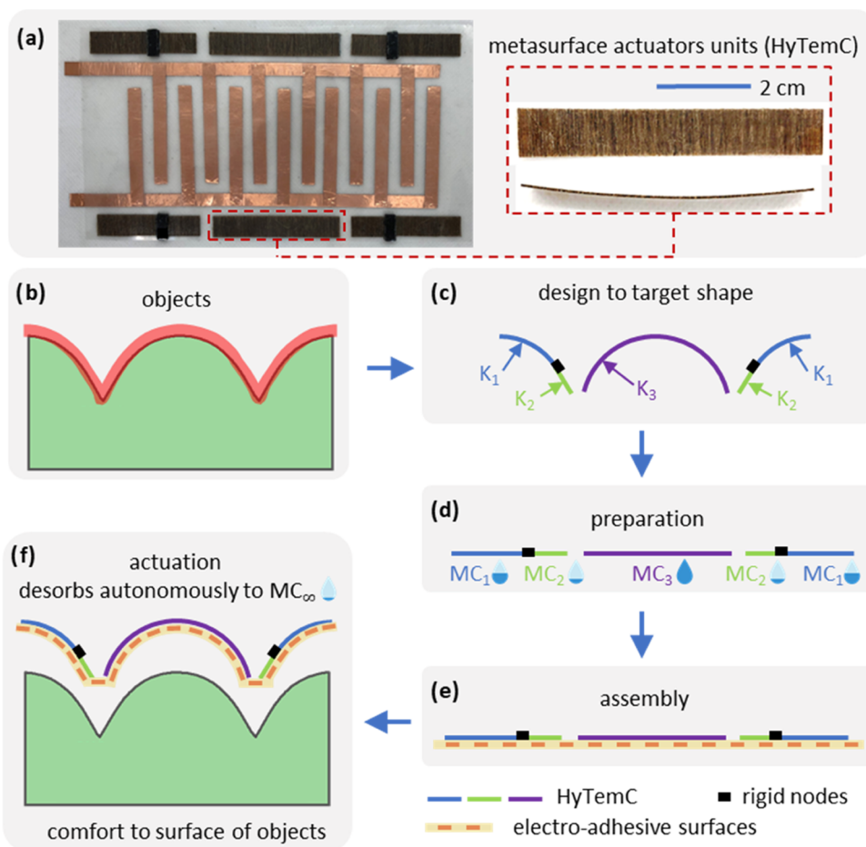
Figure 1. Demonstration of the biobased and programmable metasurface with electroadhesive capabilities (a). The electroadhesive surfaces of the objects (b) can be designed into several parts with different curvatures when considering the target surface to bond (c). The programmed biocomposite substrates are assembled to metasurfaces (d, e) with adhesive surfaces that conform to the same shapes as the target objects (f).
