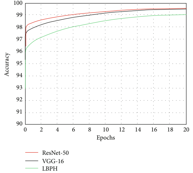
FIGURE 20: Model accuracy.
