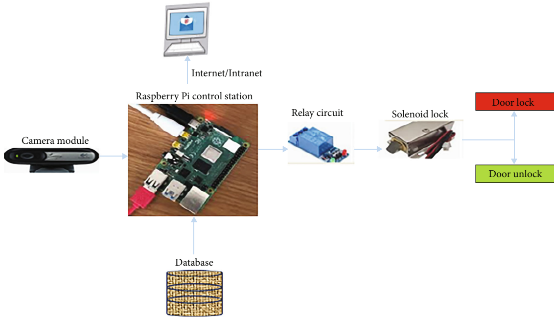
FIGURE 1: Block diagram architecture.
