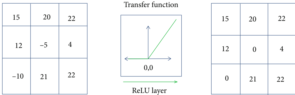
FIGURE 13: ReLU operation.
