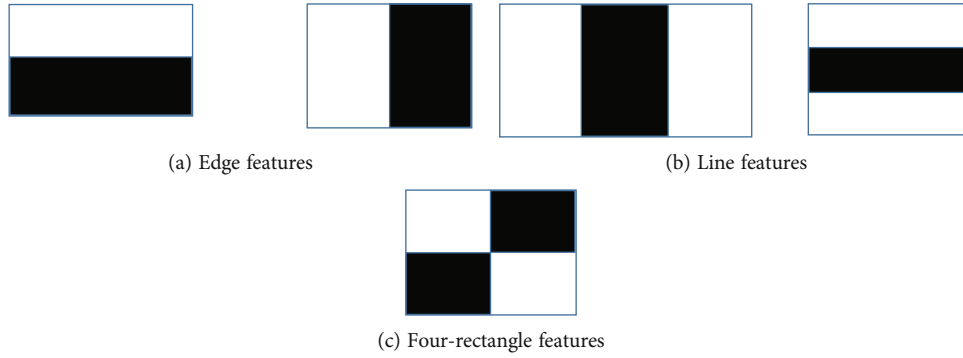
FIGURE 5: Haar features.
