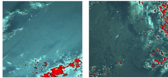
Figure 9: Cloud detection
