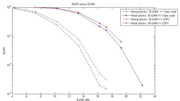
Figure 9 - 16-QAM: turbo code versus LDPC
