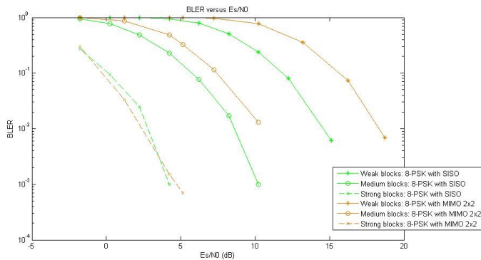
Figure 10 - 8-PSK: SISO versus 2x2 MIMO
