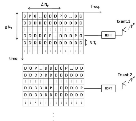
Figure 5 - frame structure for the OFDM transmitter with pilot symbols multiplexed with data (P - pilot symbols, D - data symbols, TS - lasting symbol)
