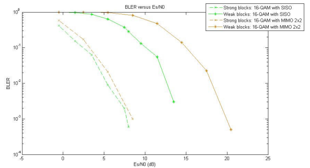
Figure 7 - 16-QAM: SISO versus 2x2 MIMO
