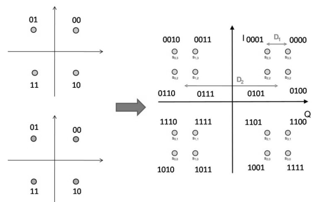
Figure 1 – construction of a 16-QAM hierarchical constellation
