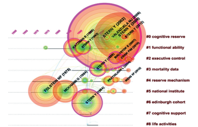
Figure 2. Timeline of co-citation clusters. Landmark articles are labeled.
