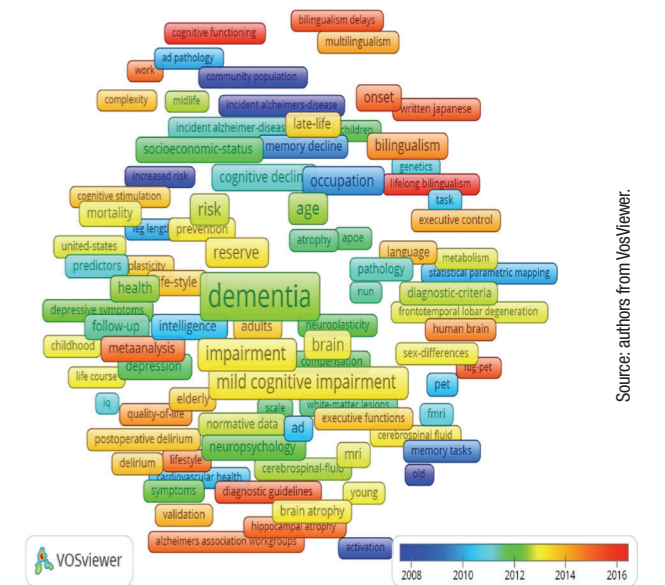
Figure 1. Network of keywords (1997-2018).
