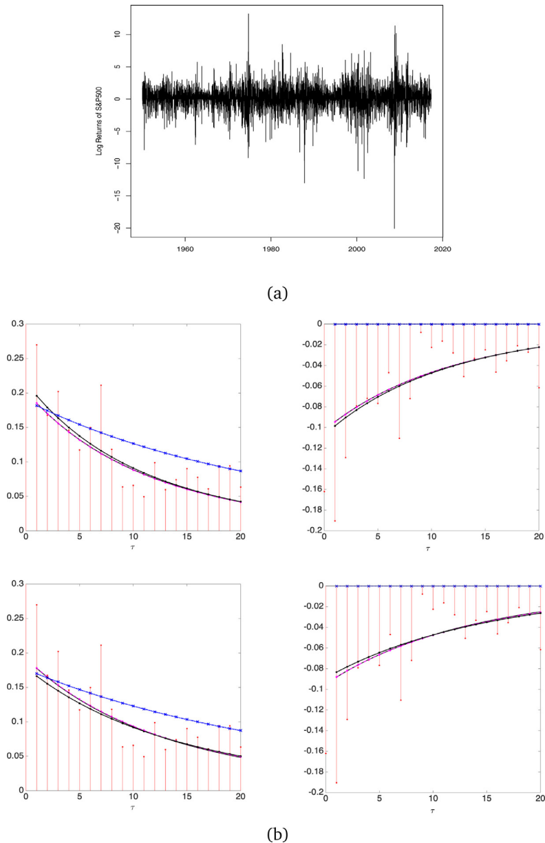
Fig. 4. (a) Weekly S&P 500 returns observed from January 9, 1950 to May 18, 2017. (b) Sample and plug-in autocorrelations (left column) and cross-correlations (right column) for the TGA-SV (solid lines), E-SV (dash lines), A-ARSV (asterisk lines) and ARSV (dash-dotted lines) models when the errors follow GED (first row) and Gaussian distributions (second row).
