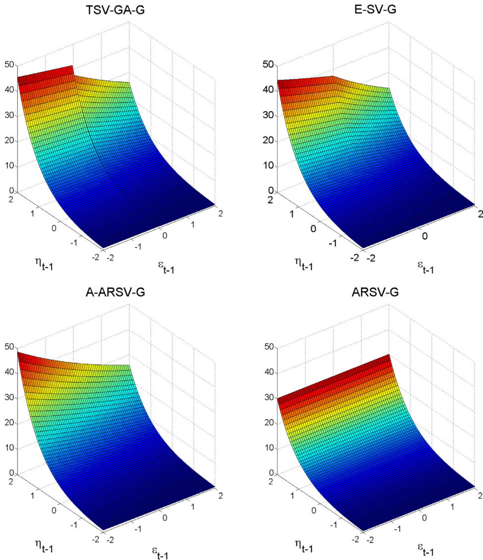
Fig. 5. Plug-in volatility responses of models with GED errors fitted to S&P 500 returns.
