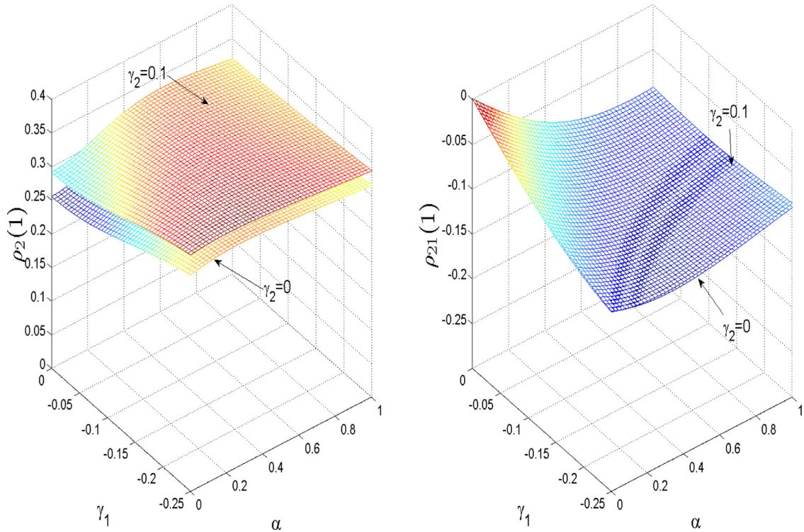
Fig. 1. First order autocorrelations of squares (left panel) and first order cross-correlations between returns and future squared returns (right panel) of different Gaussian TGA-SV models with parameters \phi = 0.98 and \sigma_{\eta}^2 = 0.05 .
