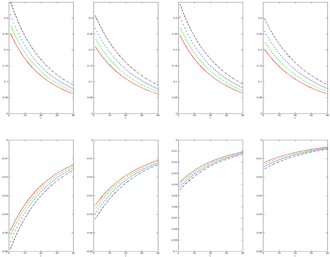
Fig. 2. Autocorrelation function of squares (first row) and cross-correlations between returns and future squared returns (second row) for different specifications of asymmetric SV models. The first column corresponds to a TGA-SV model with \alpha = 0.07 , \phi = 0.98 , \sigma_\eta^2 = 0.05 , \gamma_1 = -0.08 , \gamma_2 = 0.1 and \nu = 1.5 (solid lines), \nu = 1.7 (dashed lines), \nu = 2 (dotted lines) and \nu = 2.5 (dashdot lines). The second column corresponds to the A-ARSV model with \alpha = \gamma_2 = 0 . The third column corresponds to an E-SV model with \alpha = 0 . Finally, the last column corresponds to the RT-SV model with \gamma_1 = \gamma_2 = 0 .
