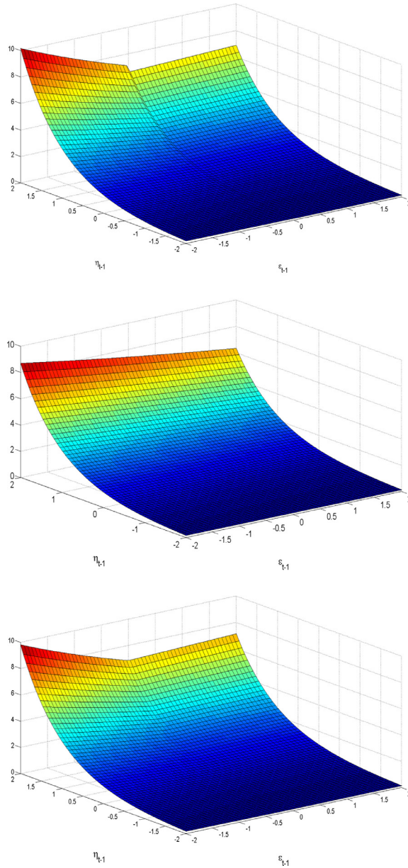
Fig. 3. Volatility responses of GA-SV models with \phi = 0.98 , \sigma_{\eta}^2 = 0.05 \exp(\mu) = 0.01 and \nu = 2 . Top panel f(\epsilon_t; \theta) = \alpha(I(\epsilon_t < 0) - 0.5) + \gamma_1 \epsilon_t + \gamma_2(|\epsilon_t| - E(|\epsilon_t|)) ; middle panel f(\epsilon_t; \theta) = \gamma_1 \epsilon_t and bottom panel f(\epsilon_t; \theta) = \gamma_1 \epsilon_t + \gamma_2(|\epsilon_t| - E(|\epsilon_t|)) . The parameter values are \{\alpha, \gamma_1, \gamma_2\} = \{0.07, -0.08, 0.1\} .
