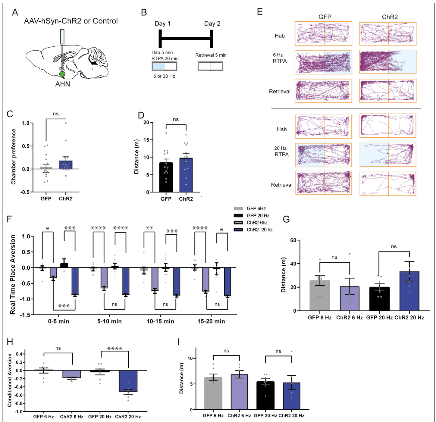
Figure 2. AHN stimulation is aversive and induces conditioned place aversion. (a) Schematic illustration of optogenetic activation in the AHN (green circle depicts the AAV infusion). (b) Schematic describing the RTPA and CPA test paradigm: day 1 consisting of habituation and real-time place preference (20 min) and day 2 for testing conditioned place preference (5 min). (c) Chamber preference during habituation (GFP N=14, ChR2 N=12, unpaired t-test, t=1.390 , df=24 , p=0.1772 , NS). (d) Distance travelled during habituation (GFP N=14, ChR2 N=12, unpaired t-test, t=0.8396 , df=24 , p=0.41 , NS). (e) Representative locomotion trajectory for a GFP control animal (left column) and a ChR2-expressing animal (right column) during habituation (hab), 6 Hz or 20 Hz real-time stimulation (6 Hz RTPA, 20 Hz RTPA), and conditioned place aversion test (Retrieval). Light-coupled chambers are shown in blue. (f) Realtime place aversion monitored across 20-min test (GFP N=7, ChR2 N=6). GFP 6 Hz vs. ChR2 6 Hz (two-way RM ANOVA, time x treatment, F(3,33)=3.965 , *p=0.016 , time effect, F(2.252, 24.77)=4.739 , p=0.152 , NS, treatment effect, F(1, 11)=77.41 , ****p<0.0001 , Sidak's multiple comparisons test, 0-5 min, *p=0.0359 , 5-10 min, ****p<0.0001 , 10-15 min, **p=0.0022 , 15-20 min, ****p<0.0001 ). GFP 20 Hz vs. ChR2 20 Hz (two-way RM ANOVA, time x treatment, F(3,33)=0.6059 , p=0.6158 , NS, time effect, F(1.938, 21.32)=1.305 , p=0.2911 , NS, treatment effect, F(1,11)=43.38 , ****p<0.0001 , 24 multiple comparisons test, 0-5 min, ***p=0.0008 , 5-10 min, ****p<0.0001 , 10-15 min, ***p=0.0007 , 15-20 min, *p=0.0127 ). GFP 6
