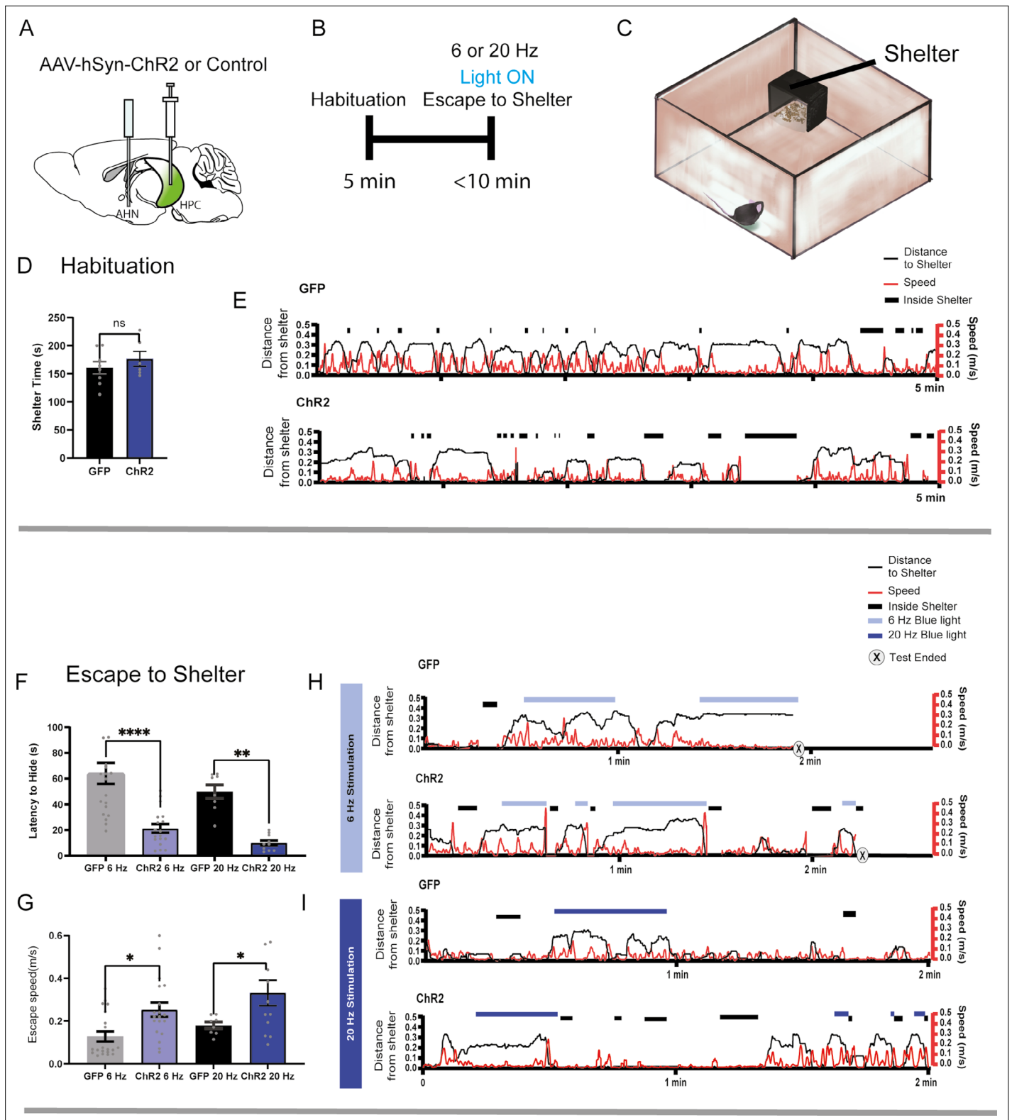
Figure 7. HPC→AHN pathway activation induces goal-directed escape. (a) Schematic illustration of optogenetic HPC terminal activation in the AHN. (b) Schematic describing a test paradigm consisting of habituation (5 min) and a 6 or 20 Hz stimulation stage to induce shelter-directed escapes. (c) A cartoon drawing of the open field arena with a shelter box. (d) Time spent in the shelter during habituation (GFP N=8, ChR2 N=6, unpaired t-test, two-tailed, t=0.9241 , df=12 , p=0.3736 , NS). (e) Representative line graphs for GFP (top) and ChR2 (bottom) mice, showing distance from shelter (black lines), speed (red lines), and moments when mice were inside the shelter (black boxes) over the 5 min habituation period. (f) Latency to escape to the
