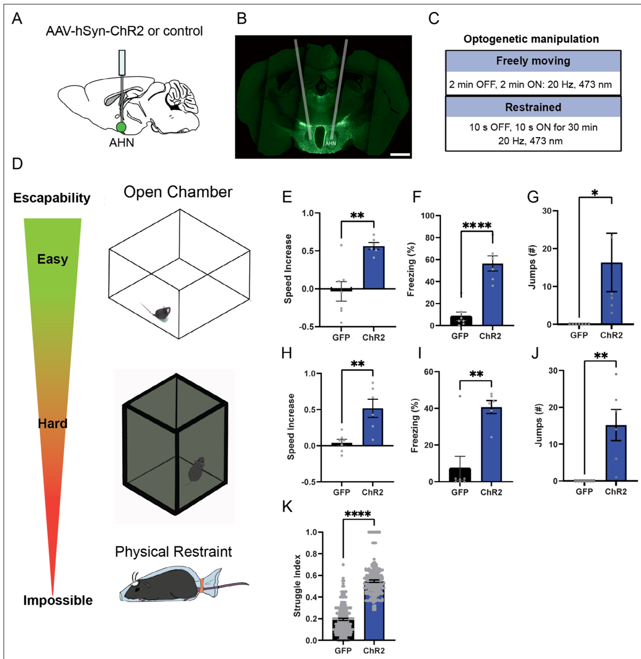
Figure 1. AHN stimulation induces escape-associated behaviors. (a) Schematic illustration of optogenetic activation in the AHN (green circle depicts the AAV infusion). (b) An example of histological confirmation showing the expression of ChR2 and placement of optic fiber in the AHN. (c) Schematic describing optogenetic stimulation paradigm. (d) Three different escape conditions where the effects of AHN stimulation was examined. Top: open field arena with short transparent walls (condition 1, easy). Middle: tall opaque walls (condition 2, hard). Bottom: physical restraint tube (condition 3, impossible). (e) Condition 1: speed increase from the light OFF epoch to ON epoch (GFP N=7, ChR2 N=6 unpaired t-test, two-tailed, t=4.119 , df=11 , **p=0.0017 ). (f) Condition 1: freezing time during the light ON epoch (GFP N=7, ChR2 N=6, unpaired t-test, two-tailed, t=6.695 , df=11 , ****p<0.0001 ). (g) Condition 1: number of jumps during the light ON epoch (unpaired t-test, two-tailed, t=2.308 , df=11 , *p=0.0414 ). (h) Condition 2: speed increase from the light OFF epoch to ON epoch (GFP N=7, ChR2 N=6, unpaired t-test, two-tailed, t=3.778 , df=11 , **p=0.0031 ). (i) Condition 2: freezing time during the light ON epoch (GFP N=7, ChR2 N=6, unpaired t-test, two-tailed, t=4.259 , df=11 , **p=0.0013 ). (j) Condition 2: number of jumps during the light ON epoch (GFP N=7, ChR2 N=6, unpaired t-test, two-tailed, t=3.796 , df=11 , **p=0.003 ). (k) Condition 3: struggle movement during the 30 min of physical restraint (GFP N=4, ChR2 N=6, unpaired t-test, two-tailed, t=26.05 , df=366 , ****p<0.0001 ). All results reported are mean \pm s.e.m. *p < 0.05 , **p < 0.01 , ***p < 0.001 , ****p < 0.0001 . Scale bar=1 mm.
