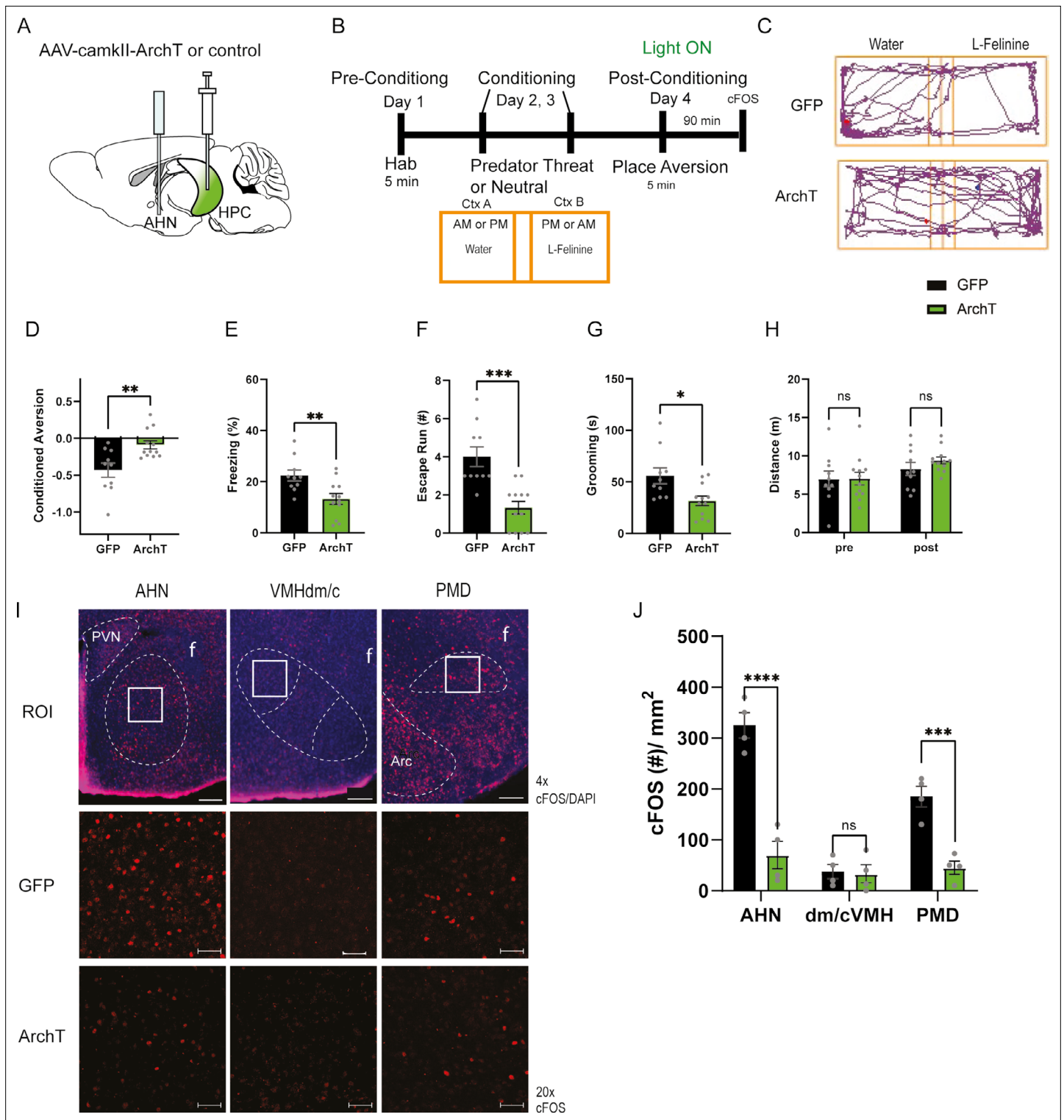
Figure 6. HPC input to the AHN is necessary for remembering the context-associated with predatory threat. (a) Schematic illustration of optogenetic HPC terminal inhibition in the AHN (GFP N=10, ArchT N=12). (b) Schematic describing the behavioral paradigm for the contextual fear conditioning with the predator odor (L-Felinine-); day 1 for habituation (5 min), days 2–3 for two daily conditioning sessions where mice were enclosed either L-Felinine- or water-paired chamber for 20 minutes in AM and PM in a counterbalanced manner, and day 4 for testing conditioned place preference (5 min) and the immunochemical detection of c-Fos. (c) Representative locomotion trajectory for a GFP control animal (top) and a ChR2-expressing animal (down) during the conditioned place aversion test with optogenetic HPC terminal inhibition in the AHN (left: water-coupled chamber, right: L-Felinine-coupled chamber). (d) Conditioned aversion memory tested 24 hr after conditioning. GFP vs. ArchT (unpaired t-test, t=3.223 , df=20 ).
