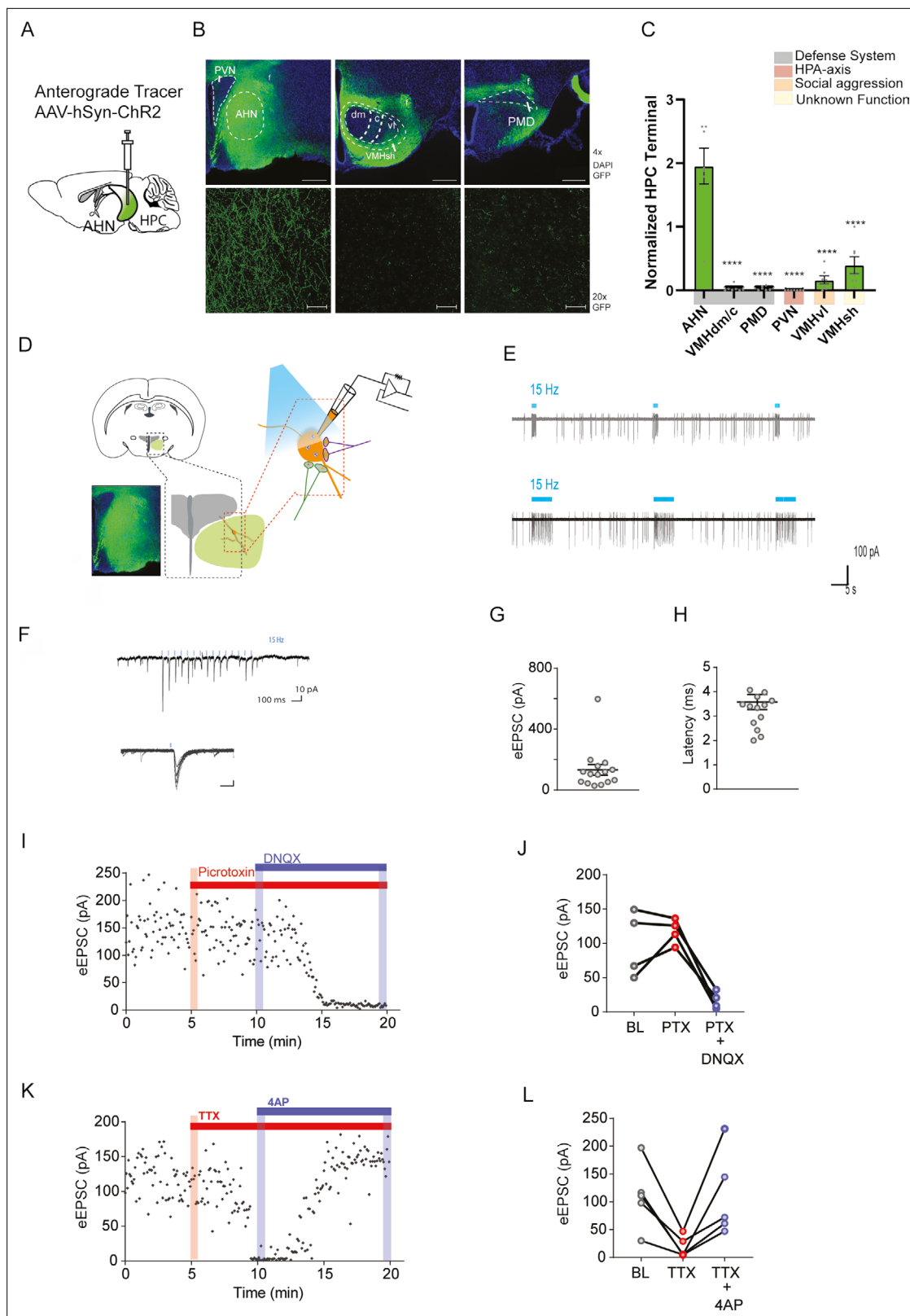
Figure 3. Hippocampus sends monosynaptic excitatory inputs to the anterior hypothalamic nucleus. (a) Schematic illustration of anterograde tracing experiment. (b) HPC terminals (green) in the hypothalamus, including anterior hypothalamic nucleus (AHN), dorsomedial and central regions of ventromedial hypothalamus (VMHdm/c), preammillary dorsal nucleus (PMD), paraventricular nucleus (PVN), ventrolateral region of ventromedial hypothalamus (VMHvl), shell of ventromedial hypothalamus (VMHsh). DAPI staining (blue). (c) Quantification of HPC terminal intensity (N=2 animals), Figure 3 continued on next page
