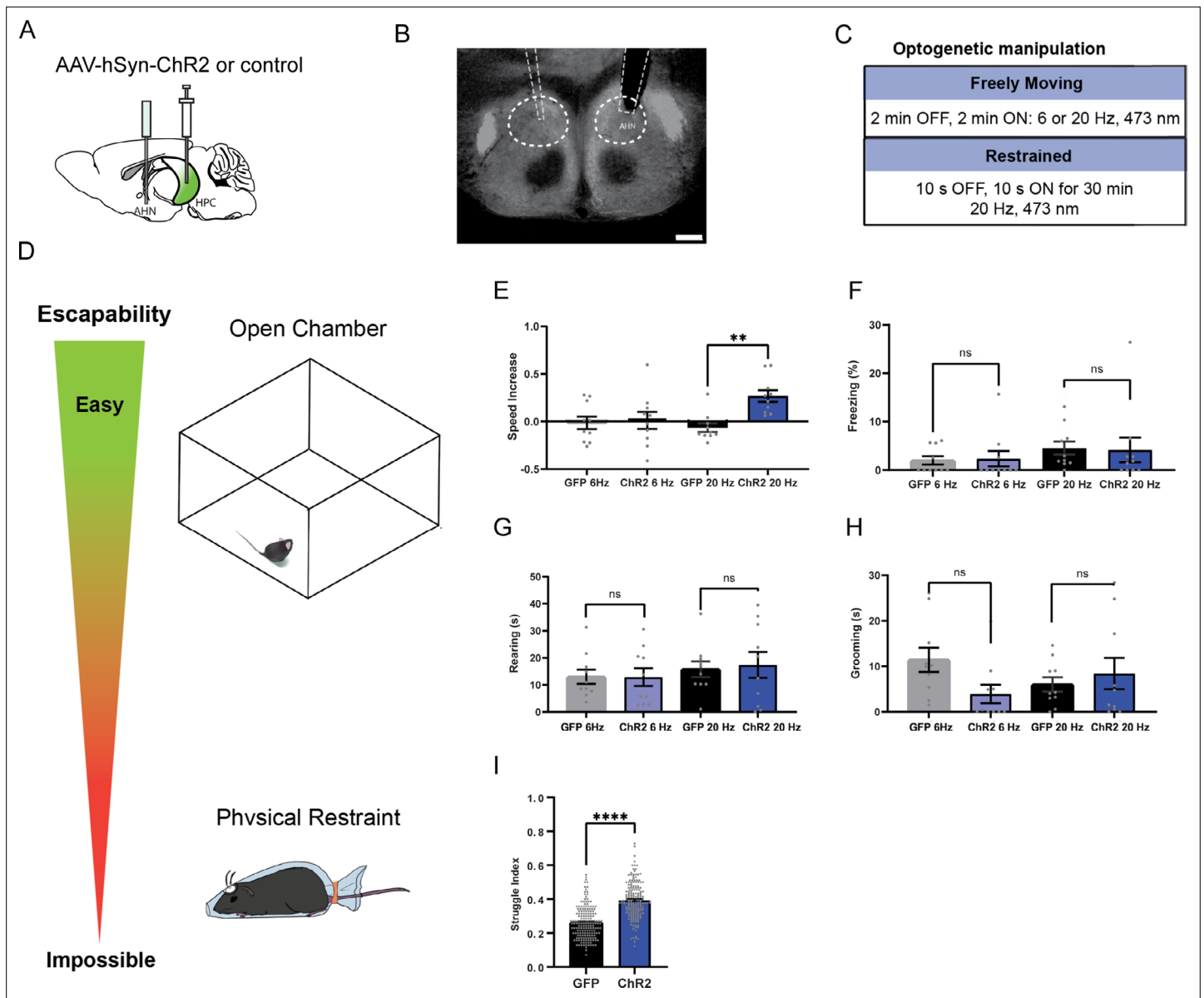
Figure 4. HPC→AHN pathway activation induces escape-associated locomotion. (a) Schematic illustration of optogenetic activation of hippocampal terminals in the AHN (GFP N=10, ChR2 N=10). (b) An example of histological confirmation showing the expression of HPC terminals and placement of optic fibers in the AHN. (c) Schematic describing optogenetic stimulation paradigm. (d) Two different escape conditions where the effects of HPC terminal stimulation was examined. Top: open field arena with short transparent walls (condition 1, easy). Bottom: physical restraint tube (condition 2, impossible). (e) Condition 1: speed increase from the light OFF epoch to ON epoch (two-way ANOVA, frequency x genotype, F(1,36)=5.298 , *p=0.0272 , frequency effect, F(1, 36)=2.337 , p=0.135 , NS, genotype, F(1, 36)=7.164 , *p=0.0111 , Sidak's multiple comparisons test, 6 Hz GFP vs. ChR2, p=0.957 , NS, 20 Hz GFP vs. ChR2, **p=0.0024 ). (f) Condition 1: freezing time during the light ON epoch (two-way ANOVA, frequency x genotype, F(1,36)=0.04839 , p=0.8273 , NS, frequency effect, F(1, 36)=1.637 , p=0.2089 , NS, genotype effect, F(1, 36) = 2.385e-005 , p=0.9961 , NS, Sidak's multiple comparisons test, 6 Hz GFP vs. ChR2, p=0.9856 , NS, 20 Hz GFP vs. ChR2, p=0.9843 , NS). (g) Condition 1: rearing time during the light ON epoch (two-way ANOVA, frequency x genotype, F(1,36)=0.06028 , p=0.8075 , NS, frequency effect, F(1, 36)=1.08 , p=0.3057 , NS, genotype effect, F(1, 36)=0.04343 , p=0.8361 , NS, Sidak's multiple comparisons test, 6 Hz GFP vs. ChR2, p=0.9996 , NS, 20 Hz GFP vs. ChR2, p=0.9375 , NS) (h) Condition 1: grooming time during the light ON epoch (two-way ANOVA, frequency x genotype, F(1,36)=3.858 , p=0.0573 , NS, frequency effect, F(1,36) = 0.03451 , p=0.8537 , NS, genotype effect, F(1,36)=1.024 , p=0.3184 , NS, Sidak's multiple comparisons test, 6 Hz GFP vs. ChR2, p=0.083 , NS, 20 Hz GFP vs. ChR2, p=0.7549 , NS). (i) Condition 2: struggle movement during the 30 minutes of physical restraint (GFP N=7, ChR2 N=9, unpaired t-test, two-tailed, t=12.22 , df=356 ****p<0.0001 ). All results reported are mean \pm s.e.m. *p < 0.05 , **p < 0.01 , ***p < 0.001 , ****p < 0.0001 . Scale bar=200 \mu m.
