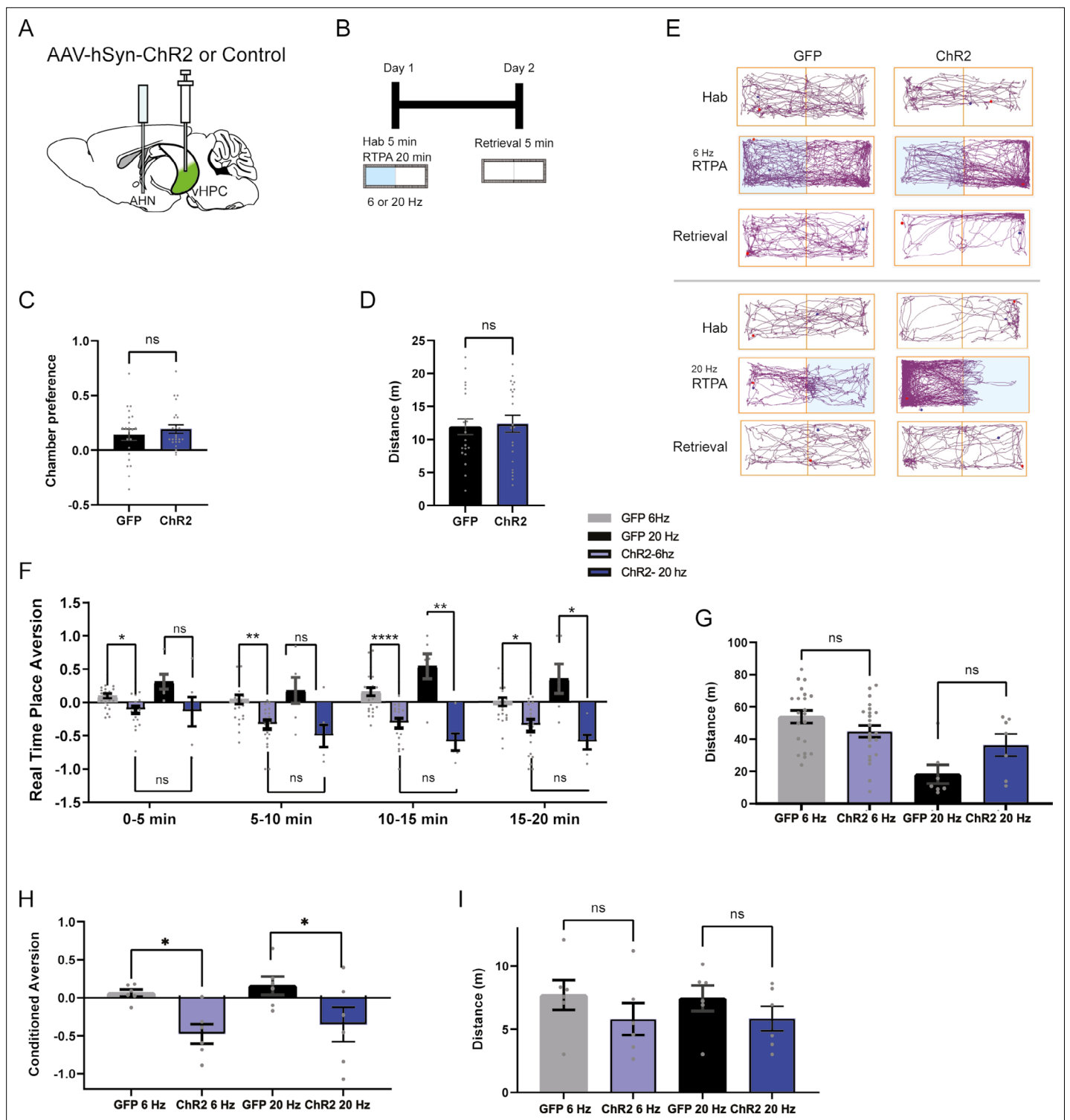
Figure 5. HPC→AHN pathway activation is aversive and instructs learning of a conditioned place aversion. (a) Schematic illustration of optogenetic activation of hippocampal terminals in the AHN (GFP N=21, ChR2 N=22). (b) Schematic describing the RTPA and CPA test paradigm: day 1 consisting of habituation and real-time place preference (20 min) and day 2 for testing conditioned place preference (5 min). (c) Chamber preference during habituation (unpaired t-test, two-tailed, t=0.8339 , df=41 , p=0.4089 , NS). (d) Distance travelled during habituation (unpaired t-test, two-tailed, t=0.2674 , df=41 , p=0.7905 , NS). (e) Representative locomotion trajectory for a GFP control animal (left column) and a ChR2-expressing animal (right column) during habituation (hab), 6 Hz or 20 Hz real-time stimulation (6 Hz RTPA, 20 Hz RTPA), and conditioned place aversion test (Retrieval). Light-coupled chambers are shown in blue. (f) Real time place aversion monitored across 20 minute test. GFP 6 Hz vs. ChR2 6 Hz (two-way RM ANOVA, time x
