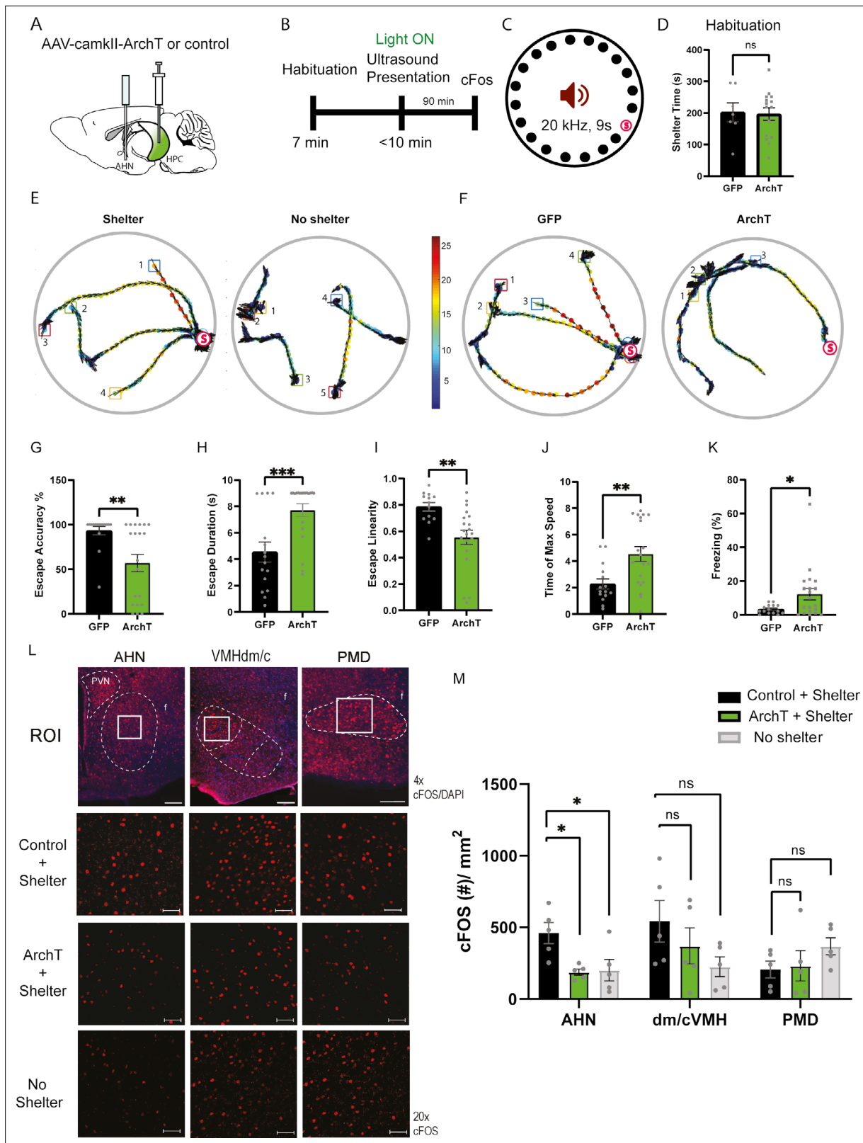
Figure 8. HPC→AHN pathway is necessary for goal-directed escape. (a) Schematic illustration of optogenetic HPC terminal inhibition in the AHN (GFP N=7 and ArchT N=15). (b) Schematic describing a test paradigm consisting of habituation (7 min) and a threat delivery stage during which ultrasound (20 kHz, 9s) is turned on after mice voluntarily come out of the shelter to induce a shelter-directed escape. (c), Top view of testing apparatus, a modified Barnes maze. ‘s’ denotes the position where a shelter was placed. The red speaker sign denotes the auditory threat played from a speaker above the
