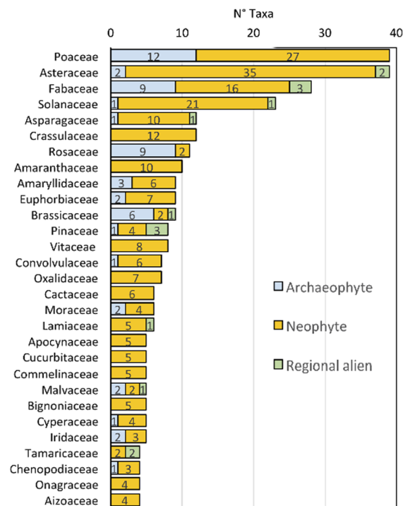
Fig. 2 The families most represented in Calabrian alien flora (≥ 4 taxa). Residence status is indicated
