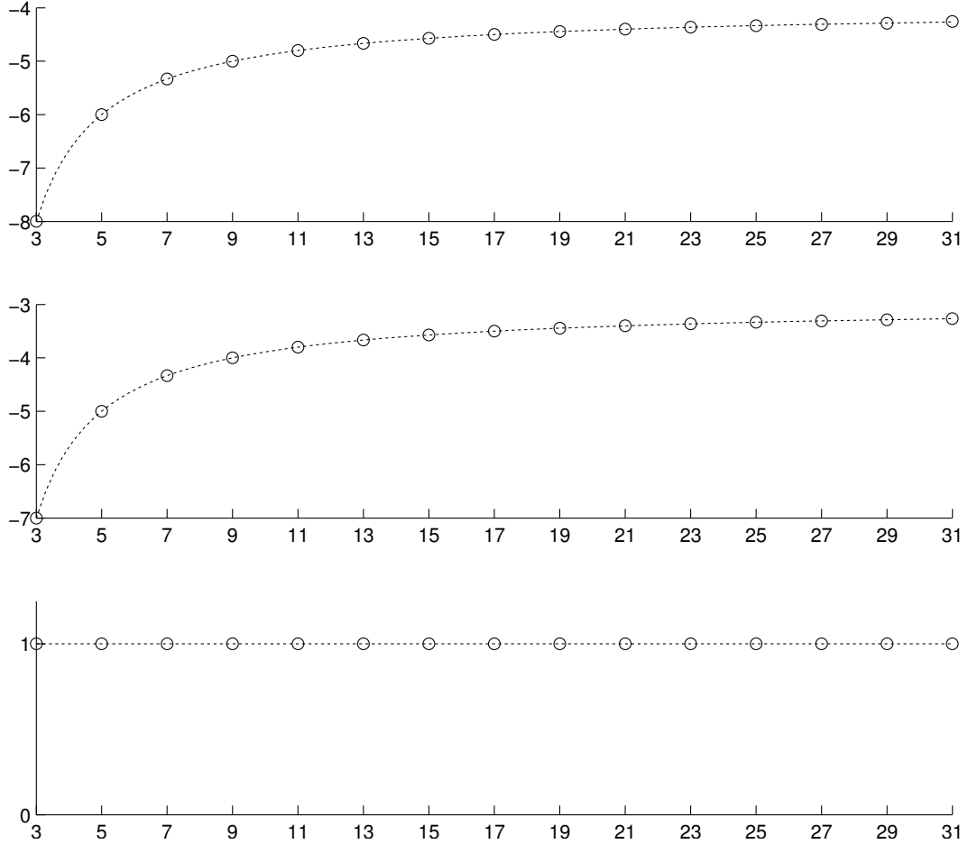
Figure 9: Numerical evidence supporting Conjecture 1 . Dotted curves represent the conjectured expression for the Floquet exponents, circles represent the result of the computations. Curves appear in the same order (top to bottom) as the exponents in the conjecture.
