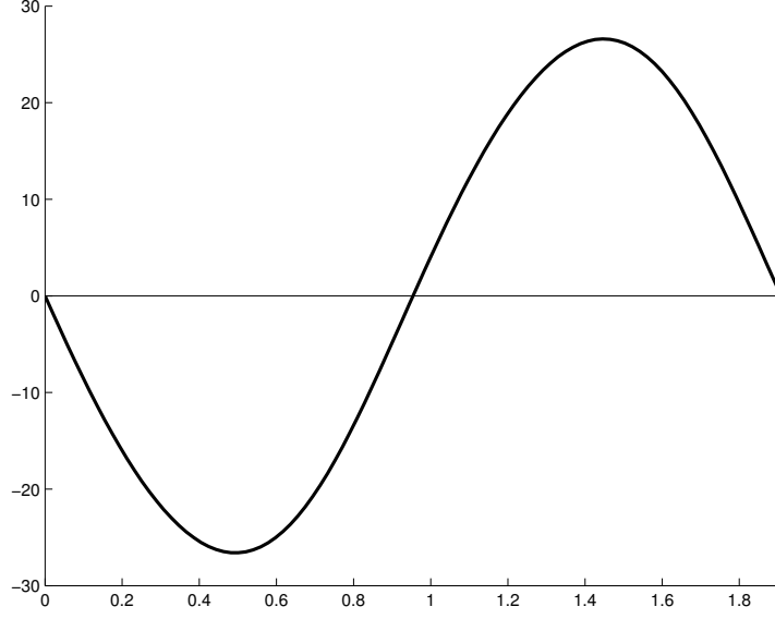
Figure 4: Graph of the periodic solution \gamma given in (4.51).
