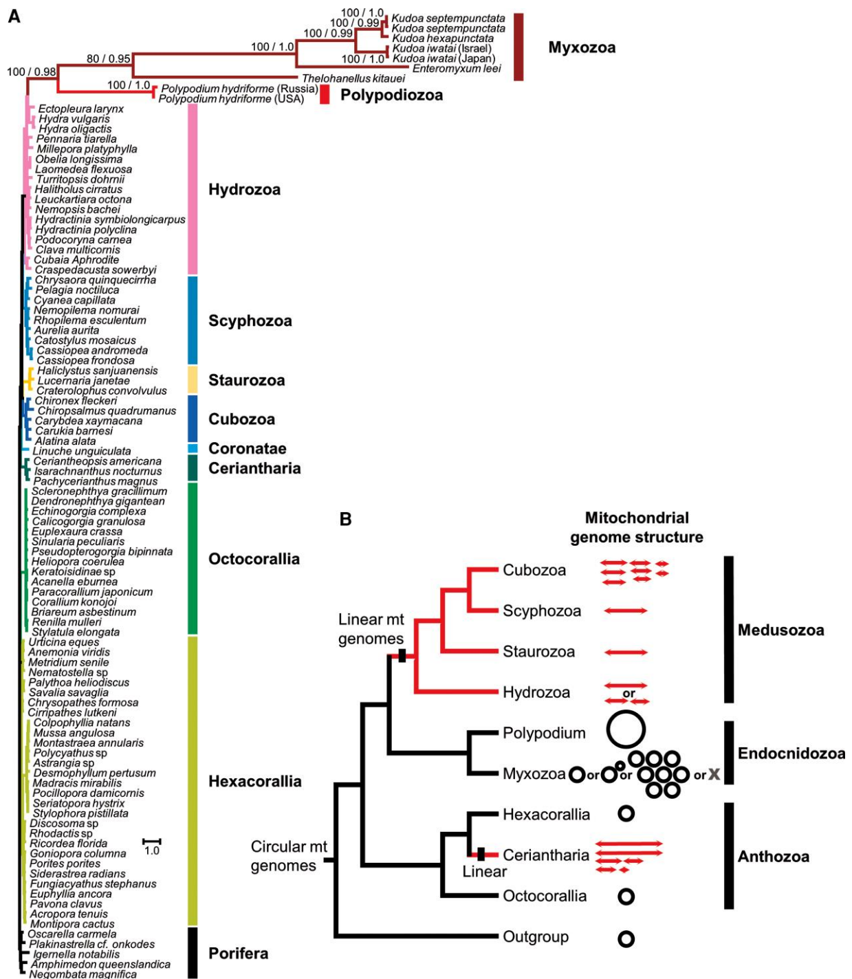
FIG. 4. —Phylogenetic analyses of cnidarian mt genomes. (A) Phylogenetic tree inferred from the concatenation of five mt proteins ( cox1 , cox2 , cytb , nad1 , nad5 ; 96 taxa and 1,700 amino-acid sites). Maximum-likelihood (ML) tree reconstructed under the LG + C60 + F + G mixture model. ML bootstrap support/and Bayesian posterior probabilities computed under the CAT+Γ mixture model are only indicated for Endocnidozoa branches (for the other branches see supplementary fig. S5, Supplementary Material online). The branch lengths exemplify the fast evolutionary rate of P. hydriforme and Myxozoa. (B) Evolution of the mt genome structure in cnidarians (based on Yahalomi et al. 2017); the topology follows Kayal et al. (2018). Red and black branches indicate linear and circular mt genomes, respectively (as illustrated by the diagrams at the end of each branch).
