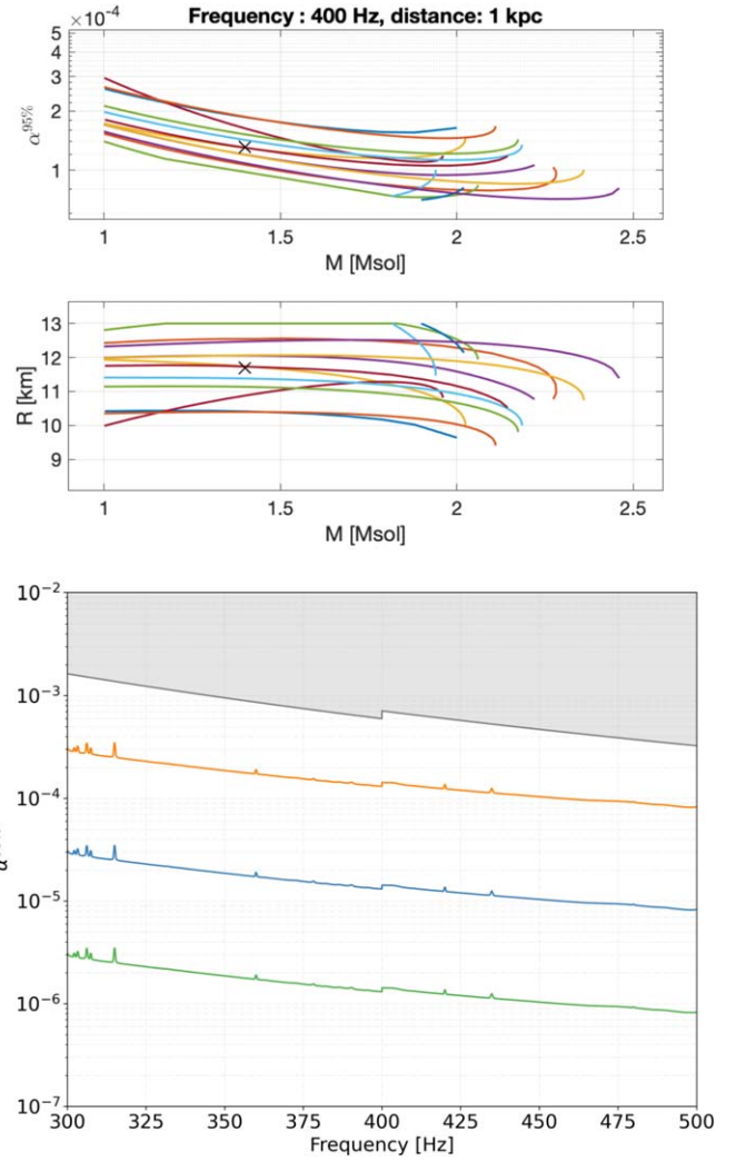
Figure 11. Upper limits \alpha^{95\%} on the r -mode amplitude at the 95% confidence level. Top plot: upper limit as a function of the neutron star mass, where we assume f = 400 Hz and a distance to the source of 1 kpc. We consider different equations of state to give an idea of the range of variability of the constraints as a function of the unknown mass and radius of the source. Middle plot: mass–radius combinations corresponding to the considered equations of state. The cross indicates the nominal mass and radius values often used of M = 1.4 M_\odot and R = 11.7 km (see Equation (9)). The equations of state are taken from Özel & Freire (2016), http://xtreme.as.arizona.edu/NeutronStars/index.php/dense-matter-eos , with M \in [1, 3] M_\odot , R \in [8, 13] km, and only ones with a maximum mass lower than 1.9 M_\odot are included (Antoniadis et al. 2013; Hebeler et al. 2013; Kurkela et al. 2014; Cromartie et al. 2019). Bottom plot: upper limit as a function of the signal frequency f_0 for sources at 1 kpc (upper orange curve), 100 pc (middle blue curve), and 10 pc (green bottom curve), having assumed M = 1.4 M_\odot and R = 11.7 km. The upper shaded gray area shows the region where this search is not sensitive.
