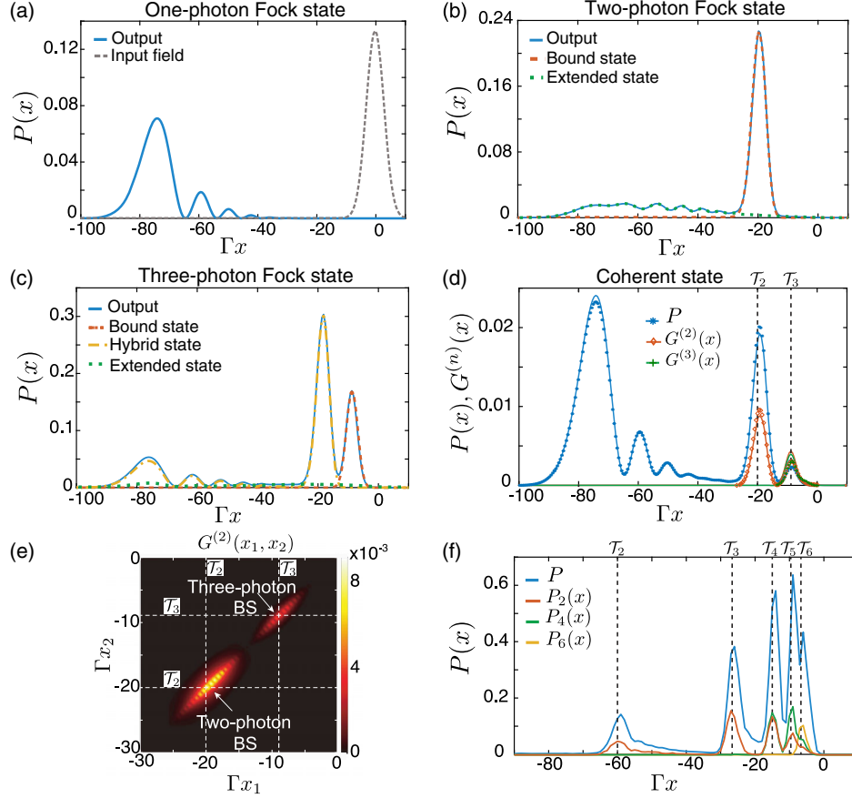
FIG. 2. Transmitted power P(x) (solid curves) for (a) one-, (b) two-, and (c) three-photon transport through N = 20 TLSs for a resonant pulse with \Gamma\sigma = 3\sqrt{2} computed using the photon-scattering theory. In (b) and (c), dashed lines show the contributions from the different eigenstates. The input mode in all panels is the Gaussian curve shown in (a). (d) Transmitted power and correlation functions for a coherent state with \bar{n} = 0.5 . Solid lines show photon-scattering results truncating at three photons, while marker points show MPS calculations performed by solving the ME with a Runge-Kutta algorithm and using maximum bond dimension D_{\max} = 150 . (e) Second-order correlation function G^{(2)}(x_1, x_2) for the transmitted coherent state computed using photon-scattering theory. The two- and three-photon bound-state contributions appear as peaks that are localized in the relative coordinate. (f) MPS calculation for input coherent state with \bar{n} = 8 , N = 60 emitters, and \Gamma\sigma = 2\sqrt{2} . Dashed vertical lines show N times the Wigner delay T_n = N\tau_n = 4N/(\Gamma n^2) . With P_n(x) , we indicate the contribution to the power coming from the emission of n photons within the space bin \Delta x = 1 . To perform this calculation, we use a quantum trajectories MPS algorithm fixing the maximum bond dimension to D_{\max} = 40 .
