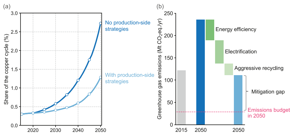
Fig. 5. GHG emissions associated with the global copper cycle, 2015–2050: (a) Share of the copper cycle in the total emissions budget for fossil fuels and industry; (b) Waterfall chart showing the extent to which different production-side strategies reduce GHG emissions from the global copper cycle in 2050. Note that since the electricity generation system is based on SSP2-RCP1.9, decarbonization of indirect emissions is already incorporated in all scenarios.
