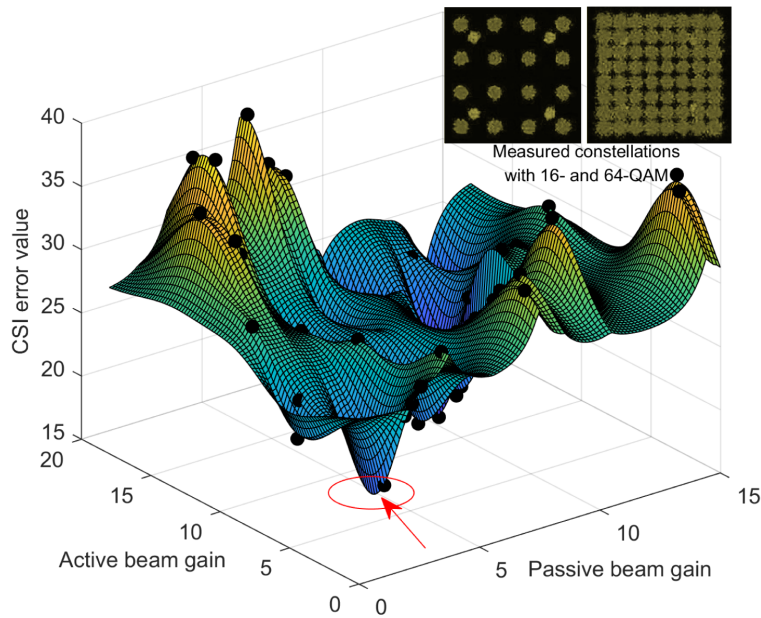
Fig. 6. Pareto front obtained as the multi-objective framework. The top right: Measured constellation plots for 16-QAM and 64-QAM data.
