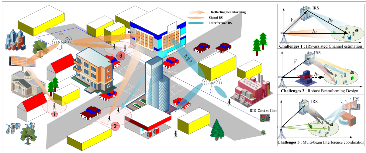
Fig. 1. Typical RIS applications in B5G/6G networks and challenges.
