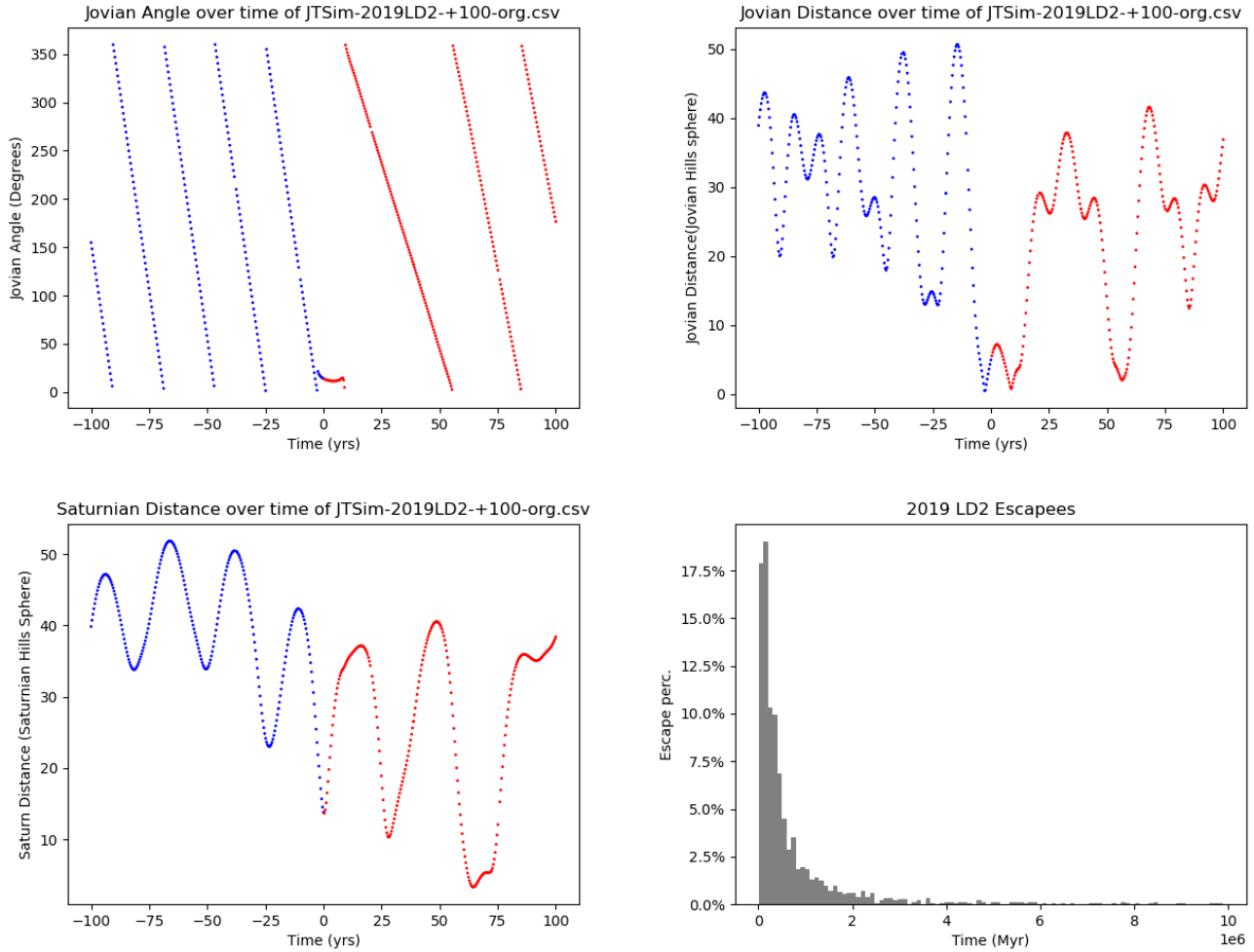
Figure 8. Top left panel: Jovian angle defined as the relative longitude between Jupiter and P/2019 LD 2 as a function of time between -100 and 100 years centered on 2019 September 15 UTC. Except for a brief period of time between -3 and 8 years where the Jovian angle was \sim 20^\circ , the Jovian angle cycled between 0^\circ and 360^\circ . Top right panel: same as the top left panel except for the Jovian distance defined as the distance between P/2019 LD 2 and Jupiter in Jovian hill spheres ( \sim 0.35 au) as a function of time. The local minimum in the Jovian distance occurred \sim 2.77 years ago with a distance of \sim 0.50 Jovian hill radius, or 0.17 au. Bottom left panel: same as the top right panel except for the Saturn distance defined as the distance between P/2019 LD 2 and Saturn in Saturn Hill spheres (0.43 au). The local minimum occurs in \sim 60 years when P/2019 LD 2 comes within \sim 3.3 Hill radii or 1.42 au of Saturn. Bottom right panel: the percentage of orbital P/2019 LD 2 clones that have escaped the Solar System (reached >1000 au from the Sun) per bin in duration of time. Each bin is \sim 100,000 years wide. Within the first million years of the simulation, \sim 78.8\% have escaped the Solar System. By 10 million years, \sim 95\% have escaped the Solar System.
