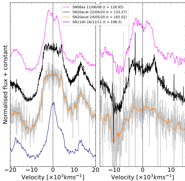
Figure 4. Comparison of the He I 1.0830 \mu\text{m} (left) and the He I 2.0581 \mu\text{m} (right) feature within the late time spectra of SN 2008ax (magenta), SN 2011dh (blue) and SN 2020acat (black and orange).
