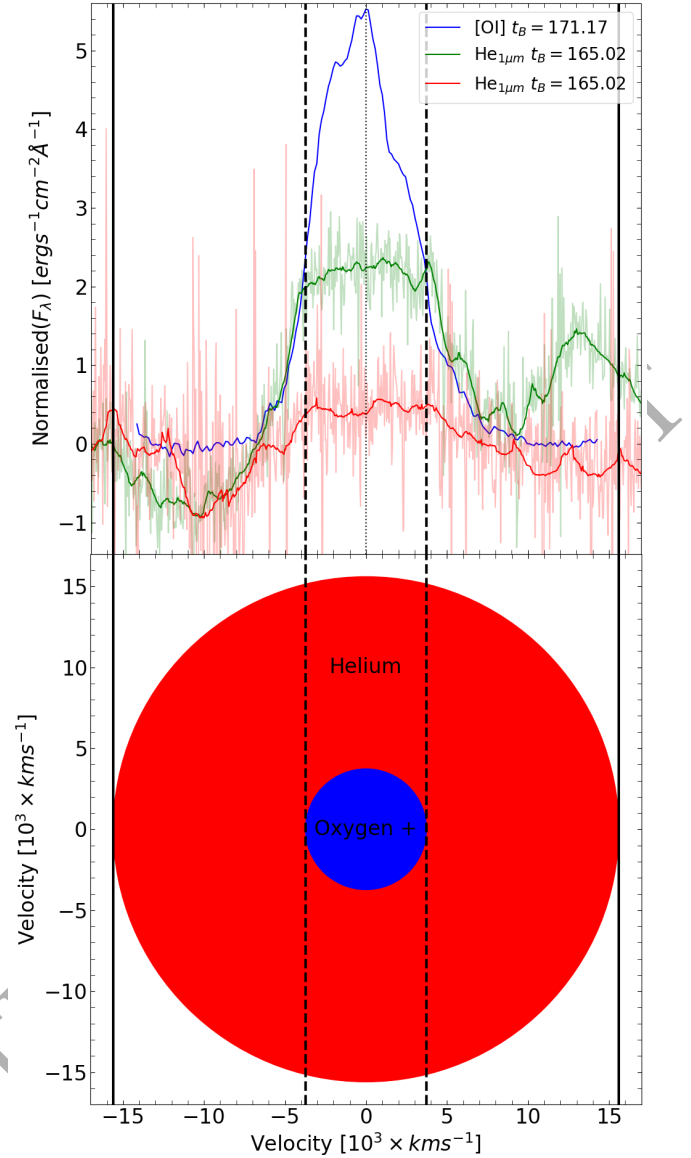
Figure 3. Top: Comparison of the late time [O I] 6300, 6363 peak and the smoothed NIR He I features. All features have been scaled to the continuum. The solid, dashed and dotted vertical lines correspond to the Helium shell v_{\text{edg}} , the FWHM of the [O I] feature and the emission wavelength of each feature respectively. Bottom: Structure of the helium and oxygen rich shells in SN 2020acat corresponding to the velocities derived from the spectra.
