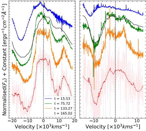
Figure 2. Velocity evolution of the He I 1.0830 \mu\text{m} and 2.0581 \mu\text{m} lines. Model fit to the day 75 spectrum (solid black line) shows a good fit to the He I 2.0581 \mu\text{m} feature. The flat-top feature of the He I 1.0830 \mu\text{m} line develops between the day 75 and 133 spectra, while the He I 1.0830 \mu\text{m} and 2.0581 \mu\text{m} line develops earlier between the day 15 and 75 spectra.
