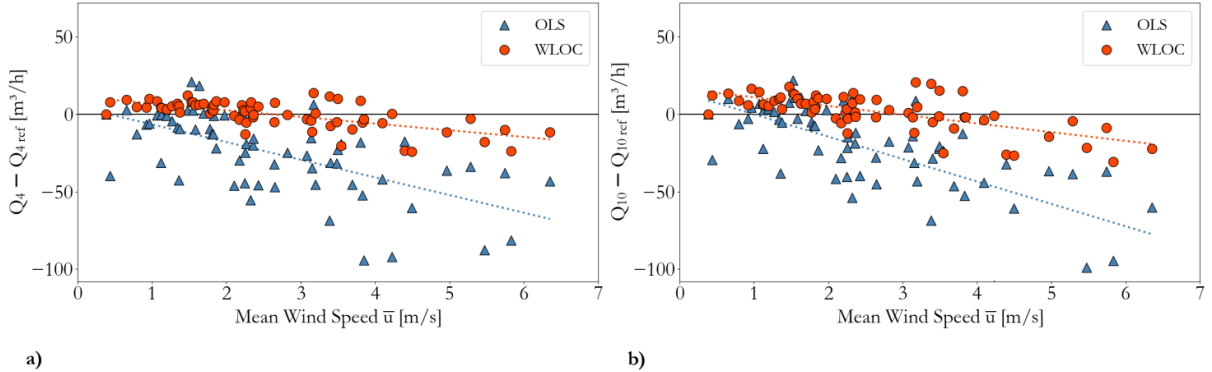
Figure 2: Relative airflow rate as a function of the mean wind speed at (a) 4 Pa and (b) 10 Pa pressure difference.
