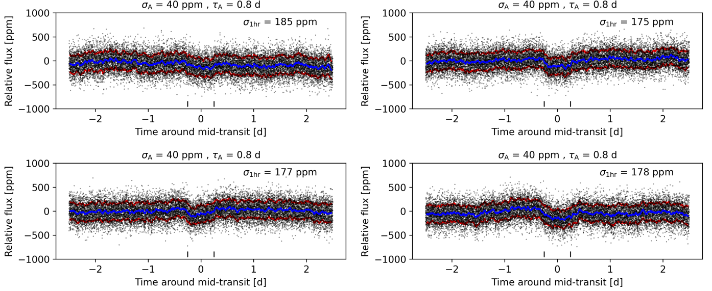
Fig. C.1. Four example light curves generated with PLS with a transit of an Earth-like planet around a solar-sized star with weak photometric activity ( \sigma_A = 40 ppm, \tau_A = 0.8 d). The light curves assumed synchronous observations with 24 PLATO cameras and m_V = 9 . The duration of the transit is indicated with two vertical black bars spanning a window of 12 hr around the mid-transit time.
