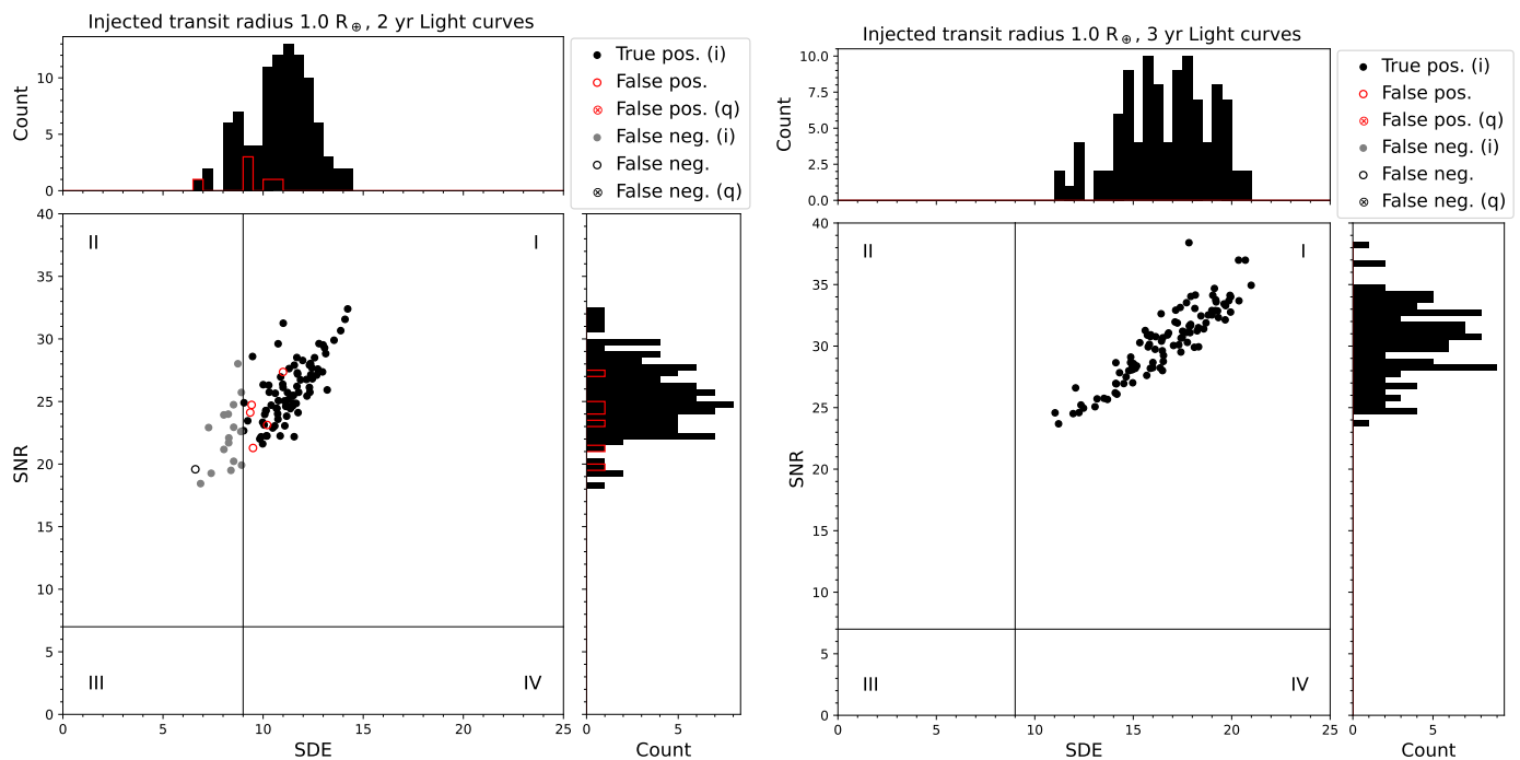
Fig. 4. Similar to Fig. 3 but now for Earth-sized planets around bright ( m_V = 8 ) Sun-like stars and 24 PLATO cameras. Panel (a) is based on two transits in 100 light curves of 2 yr length, and panel (b) shows the results for three transits in 100 light curves that are 3 yr long.
