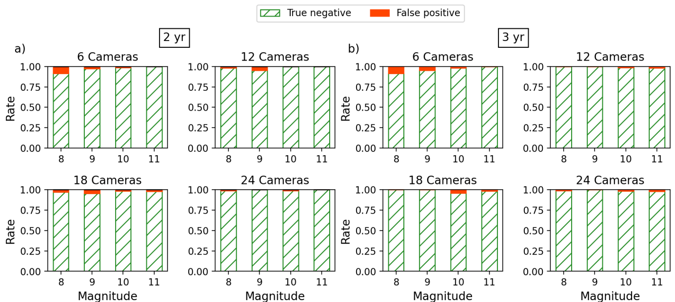
Fig. 7. Summary of our transit injection-and-retrieval experiment with PLATO-like light curves of Sun-like stars without any transiting planet. (a) Simulated light curves from PLS with a duration of 2 yr. (b) Simulated light curves from PLS with a duration of 3 yr.
