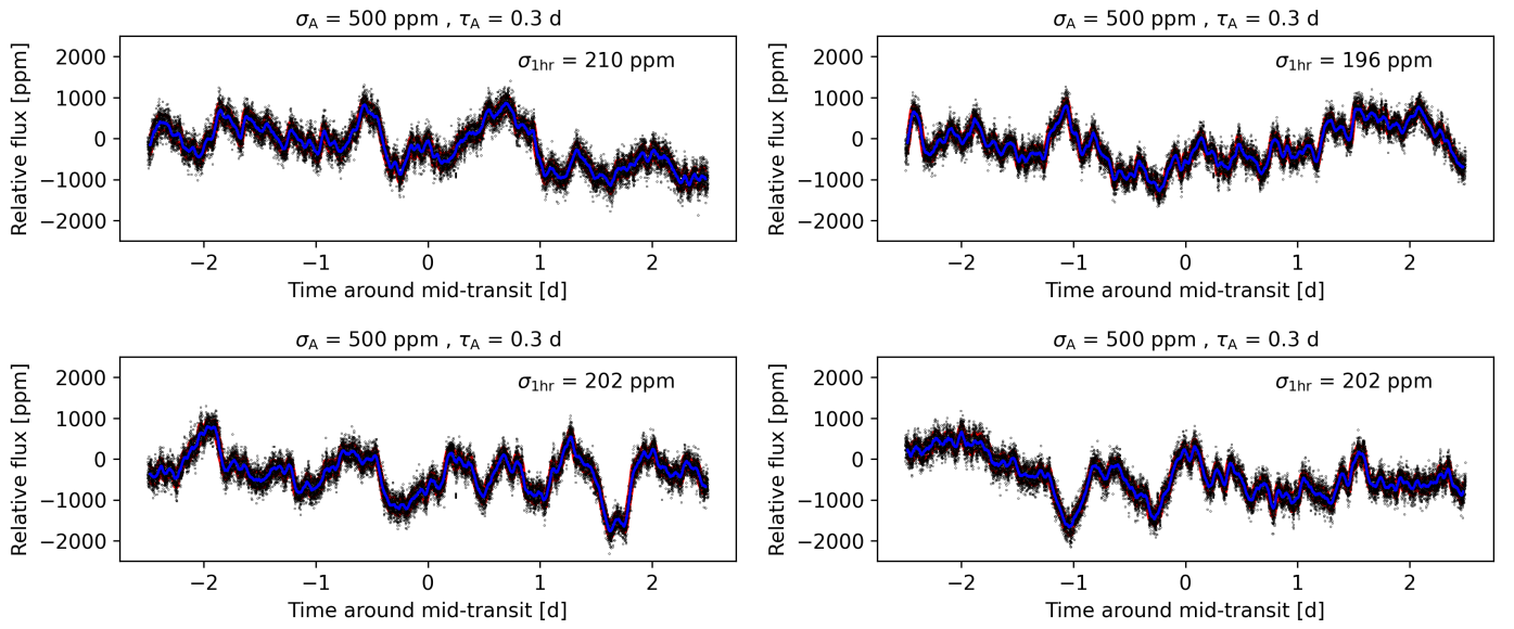
Fig. C.3. Same as Fig. C.1 but for an active star ( \sigma_A = 500 ppm, \tau_A = 0.3 d). Note the vastly different range along the ordinate compared to Figs. C.1 and C.2.
