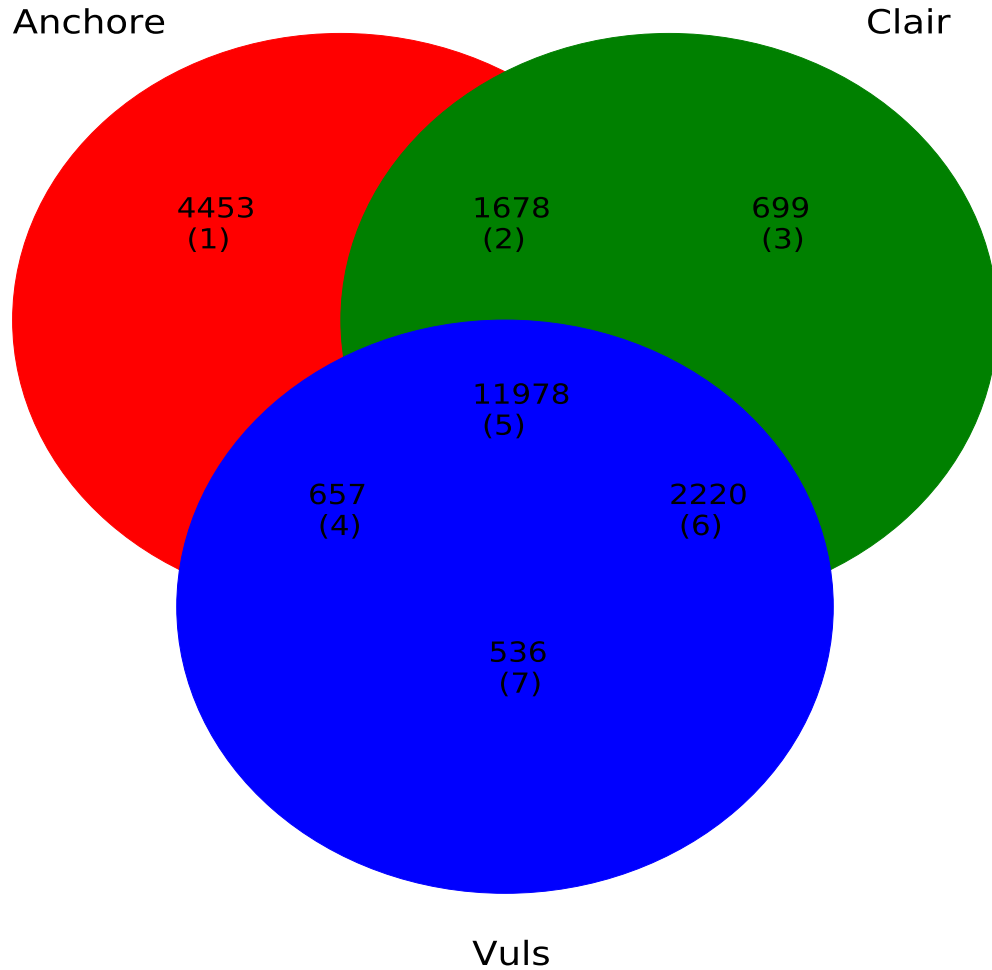
Figure 2: Differences between vulnerabilities detected by the different scanners. The Jaccard coefficients between the sets of detected vulnerabilities are quite low, showing important discrepancies between the scanners: \text{Jaccard}(\text{Anchore}, \text{Clair}) = 0.63 , \text{Jaccard}(\text{Anchore}, \text{Vuls}) = 0.59 , \text{Jaccard}(\text{Vuls}, \text{Clair}) = 0.80 . Two Ubuntu 17.04 images weren't included in this comparison as they cannot be scanned by Vuls.
