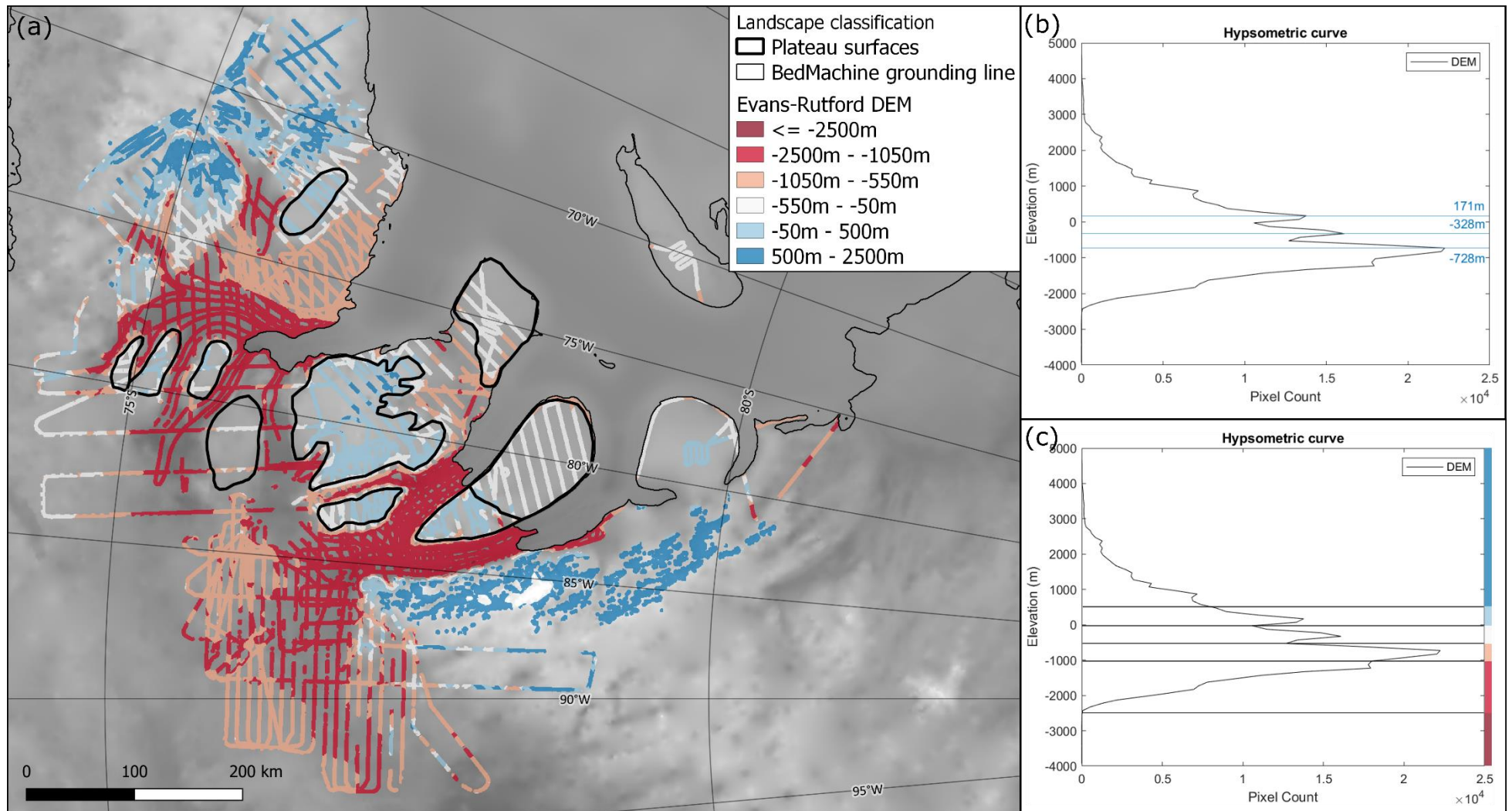
Figure 4.9: (a) Digital Elevation Model displayed in categorised symbology relating to hypsometric peaks. Plateau surfaces are outlined in black. Displayed over BedMachine subglacial topography map. (b) Hypsometric curve derived from the Digital Elevation Model with significant peak values marked. (c) Hypsometric curve classified according to significant peaks (coloured bars on right elevation scale correspond to colours in panel (a)).
