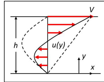
Figure 3. Couette-Poiseuille velocity profile.
