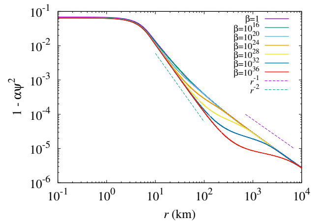
FIG. 2. 1 - \alpha \psi^2 as a function of the coordinate radius for spherical neutron stars of M_T = 1.4M_\odot . The dashed lines denote the slope of r^{-1} and r^{-2} .
