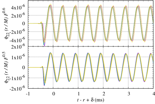
FIG. 8. The scalar waveform of \phi_{22}(r_{\text{ext}}/M)F^\eta as a function of the retarded time for \beta = 10^{28} with \eta = 0.6 (upper) and \beta = 10^{32} with \eta = 0.5 (lower). The extraction radius and the meaning of the colour are same as in Fig. 7. To align the waveforms, the plots for r_{\text{ex}} \approx 354 (green), 472 (blue), 591 (orange), and 709 km (yellow) are shifted to the positive time direction.
