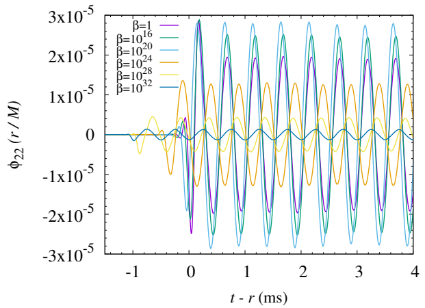
FIG. 4. Waveforms of the quadrupole mode for scalar waves as functions of t - r for \beta = 1, 10^{16}, 10^{20}, 10^{24}, 10^{28}, and 10^{32} . The waveforms extracted at r = 591 km are shown together. For \beta = 10^{28} and 10^{32} , correction factors of F^{0.6} and F^{0.5} are multiplied, respectively (see Appendix B on the correction factor).
