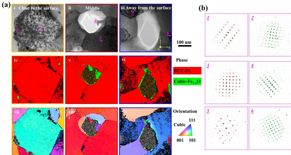
Figure 3 (A) 4D-STEM reconstruction to show (i-iii) the virtual bright-field images (iv-vi) the phase maps and (vii-ix) the orientation maps (i.e. inverse pole figure maps) of three regions
