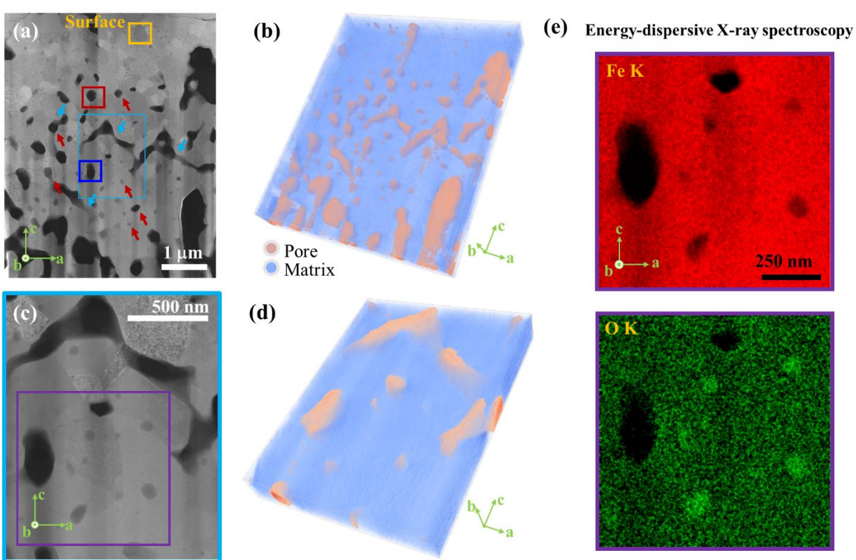
Figure 2 (a) A representative HAADF image of the H-reduced cubic- \text{Fe}_{1-x}\text{O} sample. Areas marked with red arrows appear to assume a faceted Wulff shape. Regions of interest for 4D-STEM scans (Fig. 3) are outlined in color. The rectangular areas in orange, red, and blue are regions close to the surface, in the middle of the lamella, and away from the surface, respectively. Some channels between adjacent pores are marked by blue arrows. (b) 3D reconstruction of the ET results. The regions in royal blue color coding are the BCC-Fe matrix, while the salmon-colored ones are the pores. The reconstruction is based on 29 HAADF images (tilting from -70^\circ to 70^\circ for every 5^\circ ).
