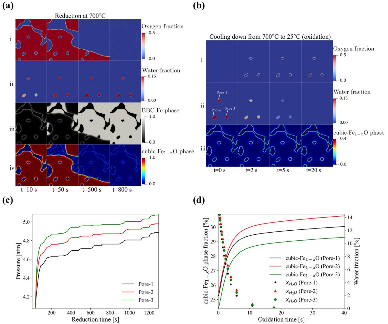
Figure 4 (a) i-iv top-to-bottom rows show the phase field simulation results for the molar fraction of oxygen and water, and the BCC-Fe phase and cubic- \text{Fe}_{1-x}\text{O} phase fractions, respectively, at different reduction time at 700°C. (b) i-iii Contour plots of the oxygen and water content, and cubic- \text{Fe}_{1-x}\text{O} phase evolution at different oxidation times during the cooling process from 700°C to 25°C. Since the cooling time is comparatively small, the oxidation reaction rate is treated as constant. (c) Pressure change of different pores under the reduction reaction at 700°C. (d) Fractions of water vapor and of the cubic- \text{Fe}_{1-x}\text{O} phase fraction of different pores during the simulated cooling, the initial number of the cubic- \text{Fe}_{1-x}\text{O} is based on the final status of the reduction process, and the initial water fraction is around 15% which is the equilibrium one in reduction.
