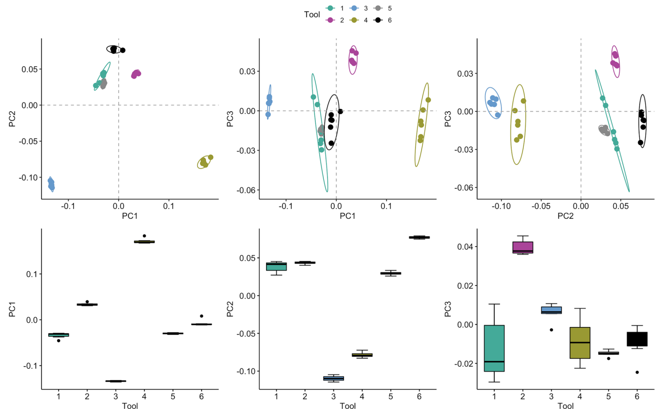
Fig. 6 Scatterplots (top row) and boxplots (bottom row) of repeat capture scores along principal components (PC) 1–3, demonstrating the clustering within tools (1–6). PC1 represents 59.7% of the total variance, whilst PC2 and PC3 account for 33.4% and 3%, respectively
