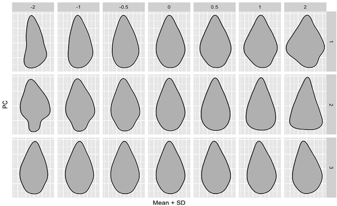
Fig. 5 Principal component (PC) contributions along the first 3 axes of variance within the multiple observer outline data
