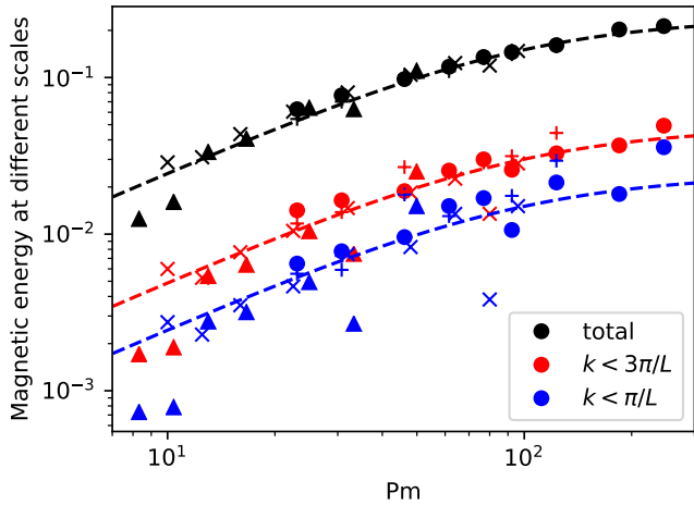
Figure 5. Magnetic energy contained in the largest scales of the box as a function of the magnetic Prandtl number. Blue and red symbols correspond to the energy at wavenumbers smaller than \pi/L and 3\pi/L respectively, while black symbols show the total magnetic energy. The symbol shapes correspond to different Reynolds numbers as in Fig. 1: Re = 400 (circles), Re = 800 (crosses) and Re = 1600 (triangles). The low resolution tests at Re = 400 are represented with the plus signs. The dashed lines represent the fit of the total magnetic energy (black), and a fraction of 20% (red) and 10% (blue) of this fit, respectively.
