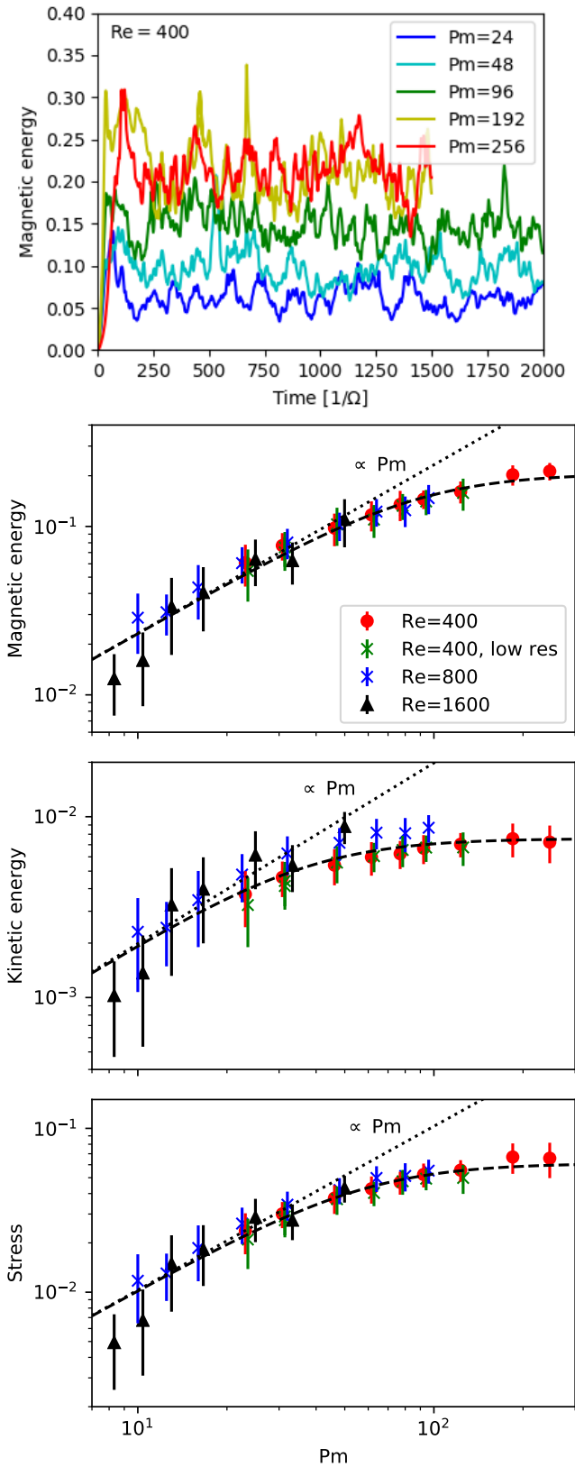
Figure 1. Top panel: Time evolution of the magnetic energy for a subset of simulations with Re = 400 and Pm \in [24, 256] . Lower panels: Time and volume averaged magnetic energy ( E_{\text{mag}} \equiv B^2/2\mu_0 ), kinetic energy ( E_{\text{kin}} \equiv v^2/2 ) and stress ( \alpha \equiv \rho_0 v_x v_y - B_x B_y / \mu_0 ) as functions of the magnetic Prandtl number for three different values of the Reynolds number Re = 400 (red circles), Re = 800 (blue crosses) and Re = 1600 (black triangles). The error bars show the standard deviation, which probably overestimates the actual error on the averages. The dotted line shows a linear fit valid at moderate Pm , while the dashed line shows the fit with Eq. 5. The stress and energies are in units of \rho_0 L^2 \Omega^2 (with L the radial size of the box).
