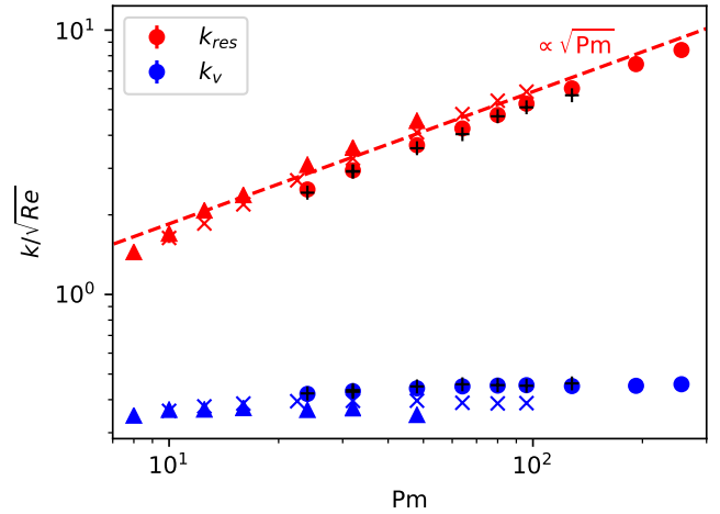
Figure 4. Typical wavenumbers of the resistive dissipation (red symbols, defined such that half of the resistive dissipation takes place at higher/lower wavenumber) and of the kinetic energy (blue, defined such that half of the kinetic energy is located at higher/lower wavenumbers). The wavenumbers have been normalised by \sqrt{Re} so that the dependence on the Reynolds number is approximately scaled out. The symbol shapes correspond to different Reynolds numbers as in Fig. 1: Re = 400 (circles), Re = 800 (crosses) and Re = 1600 (triangles). The low resolution tests at Re = 400 are represented with the black plus signs. The dashed line represent a scaling of the resistive wavenumber as \propto \sqrt{Pm} .
