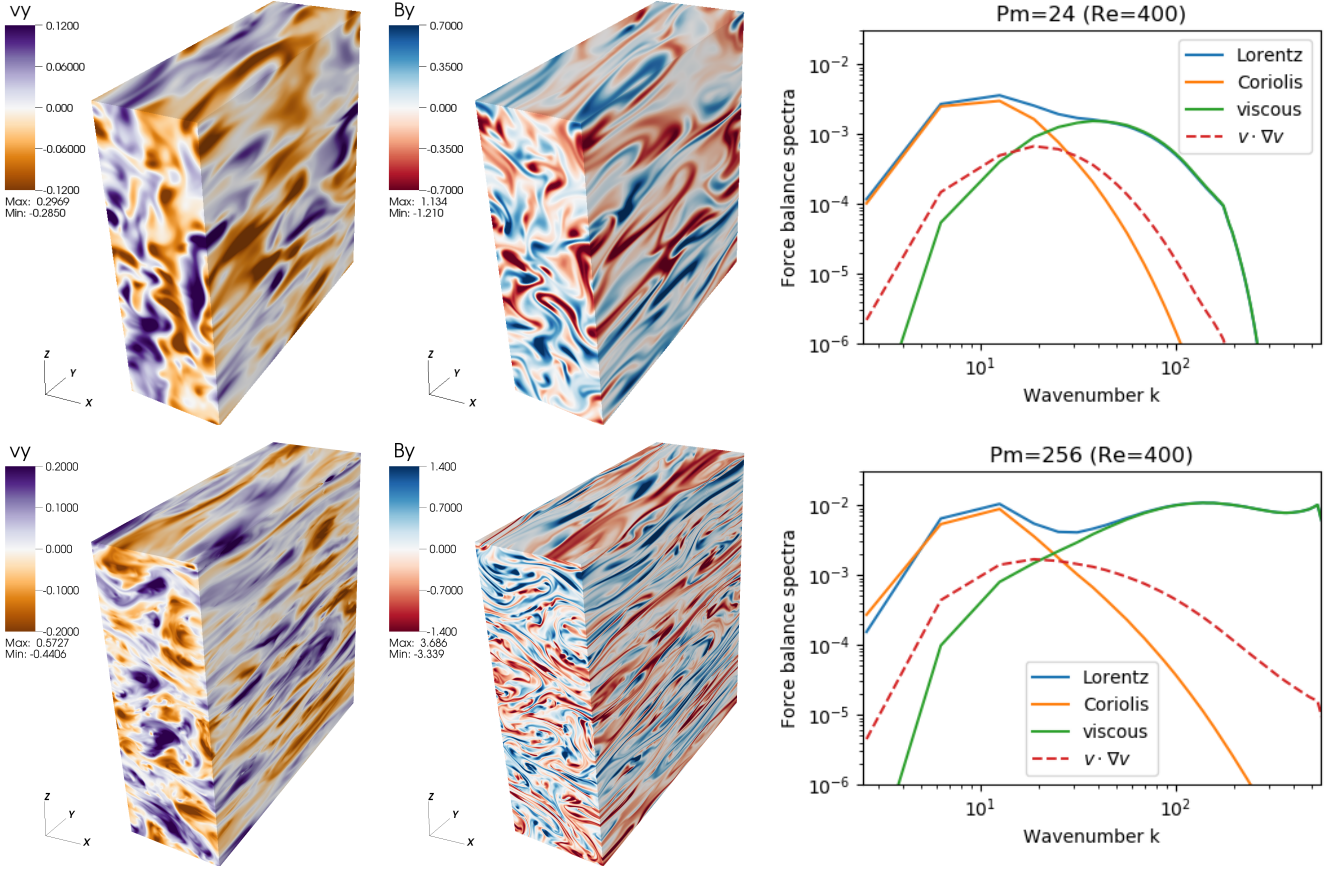
Figure 2. 3D rendering of the azimuthal component of the velocity field (left panels) and of the magnetic field (middle panels). The right panels represent the time-averaged spectra of the force balance. The upper row corresponds to a simulation with a moderate value of Pm = 24 , while the lower row corresponds to a large value of Pm = 256 . Both simulations share the same Reynolds number Re = 400 . In the force balance spectrum, only the divergence-free part of the forces is included as it is appropriate in the incompressible approximation.
