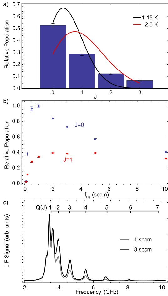
Figure 13. (a): Distribution of the AlF population over the four lowest rotational levels in the vibrational ground state of the X 1 Σ + state. The solid lines show Boltzmann distributions at 1.15 K and 2.5 K, respectively. (b): Influence of the helium buffer gas flow rate f_{\text{He}} on the fluorescence signal in LIF-2, detected on the R(0) line (blue) and the R(1) line (red). (c): Q-branch scans at He buffer gas flows of 1 sccm and 8 sccm.
