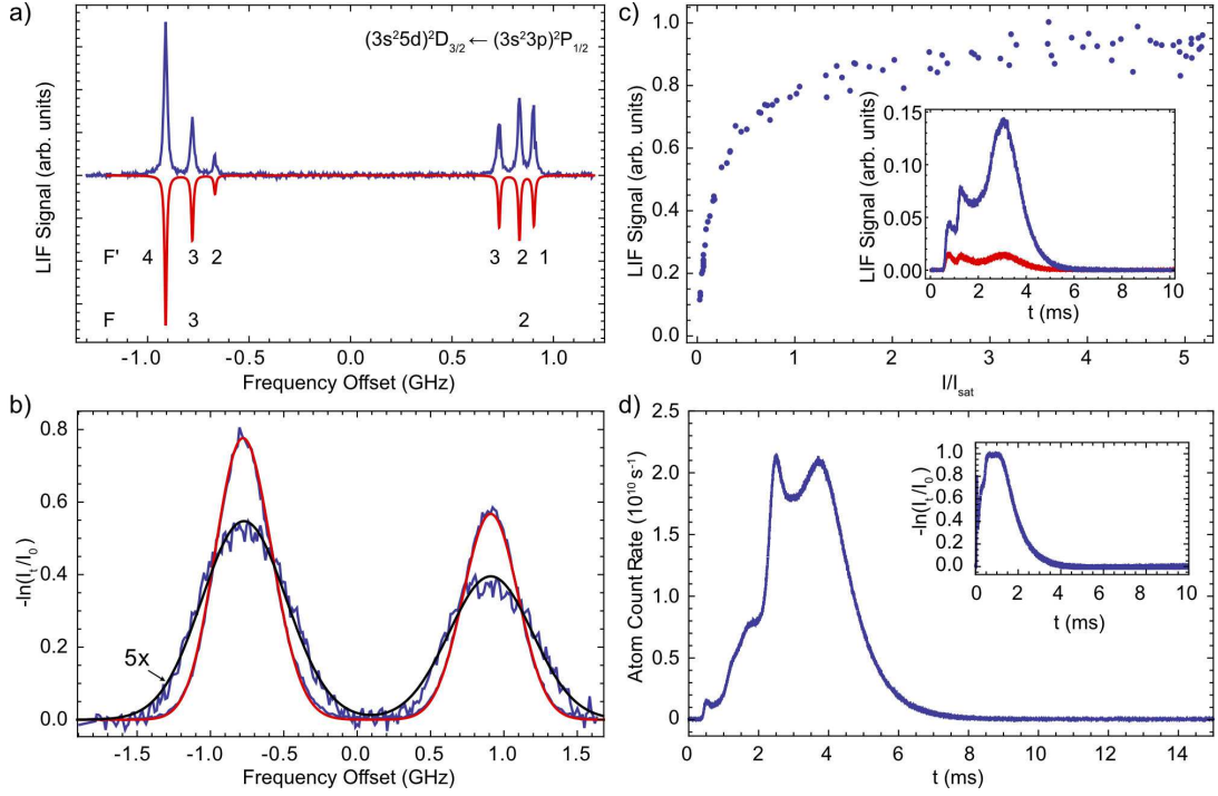
Figure 4. (a): Hyperfine-resolved LIF spectrum of the (3s^25d)^2D_{3/2} \leftarrow (3s^23p)^2P_{1/2} transition of Al near 227.6 nm. The experimental spectrum is shown in blue. A simulated spectrum using equations 7 and 8 and the known linewidth of 12.8 MHz is shown in red. The ground-state ( F ) and excited-state ( F' ) hyperfine quantum numbers of the transitions are given below the simulated spectrum. (b): Aluminium absorption spectra recorded directly outside the cell exit and 10 mm downstream (magnified by a factor five). The solid curves in red and black are fits to the data (blue) using the known spectroscopic constants and a Gaussian lineshape to determine the Doppler broadening. The Doppler broadening increases for the downstream position. (c): Fluorescence saturation curve of the (3s^25d)^2D_{3/2}, F' = 4 \leftarrow (3s^23p)^2P_{1/2}, F = 3 line of Al, demonstrating that we can saturate the fluorescence by optical pumping. The inset shows the LIF TOF without (blue) and with (red) a pumping laser on the same transition in LIF-1. (d): Time of flight traces of the Al beam under saturated fluorescence of the (3s^25d)^2D_{3/2}, F' = 4 \leftarrow (3s^23p)^2P_{1/2}, F = 3 transition to determine the total flux through a 2 \times 2 mm 2 aperture 440 mm from the source aperture. The inset shows the absorption trace directly outside the cell.
