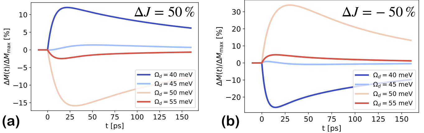
FIG. 10. Magnetization dynamics for frequencies below and above resonance. (a) For a transient increase in J of 50% ferromagnetism should increase in equilibrium, however in the presence of a high-frequency drive this can amplify, diminish, or even reverse as the frequency passes through resonance with the bath. For \Omega_d = 40 meV the relaxation rate reaches near maximal enhancement and the magnetization is most responsive to the pump-induced increase in J , while for \Omega_d = 50 meV it has already passed to the other side of the resonance. The bath now acts to induce “gain” rather than loss and drives the magnetization opposite to the naive result, quite dramatically. (b) If we consider instead a pump-induced reduction in J of =50\% the same features qualitatively persist, with opposite directions. In this case, driving above the resonance leads to a substantial enhancement of magnetization.
