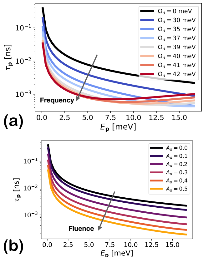
FIG. 8. (a) Plot of magnon lifetime \tau_{\text{p}} = 1/\gamma_{\text{p}} in the presence of the coherent phonon enhancement as a function of magnon kinetic energy E_{\text{p}} for different drive frequencies. We fix fluence parameter A_d = .3 and fix orbital parameters to \Delta = 90 meV and \Gamma = 10 meV, with \lambda = 15 meV. The lifetime is reduced by the magnon appearance of sidebands at \Delta \pm 2\Omega_d . Near \Omega_d = 40 meV this process nears resonance and the decay rate is maximally enhanced by nearly two orders of magnitude. (b) We study for varying drive fluence parameter A_d at fixed \Omega_d = 35 meV for the same orbital parameters. The dependence in this model is monotonic, though in a more refined model we would expect some saturation as A_d \rightarrow 1 .
