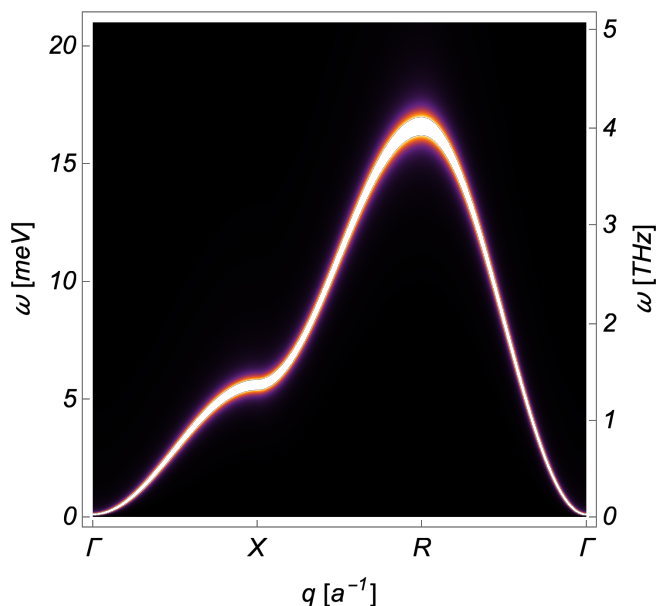
FIG. 4. Magnon spectral function A_{\text{mag}}(\omega, \mathbf{p}) = -\frac{1}{\pi} \Im G^R(\omega, \mathbf{p}) including orbital bath for N_{+-} = .5 , \lambda = 15 meV, \Delta = 90 meV, and \Gamma = 10 meV. Plotted along same dispersion contour as Fig. 3. Damping is approximately proportional to frequency, so that the linewidth \gamma_{\mathbf{p}} \sim \Omega_{\mathbf{p}} . The Lamb shift due to the orbital bath is renormalized away so that the magnon gap is the physically measured gap of \Omega_0 = 0.1 meV.
