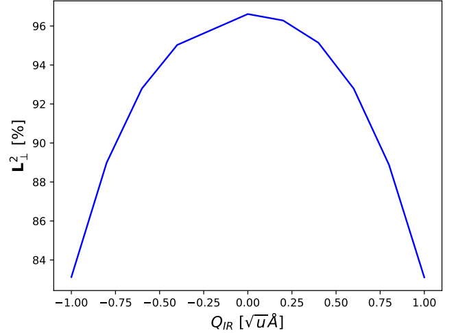
FIG. 6. Change in in-plane projection of angular momentum unit vector \mathbf{n}_j for 9 THz B_{2u} polarized phonon mode in YTO. We expect for realistic fluence, the peak amplitude is of order 1 in these units, leading to an appreciable change in the eigenvalues of the anisotropy tensor \mathbb{N} which oscillate at frequencies \pm 2\Omega_d . This motivates the amplitude parameter A_d of order A_d \sim \sqrt{.1} = .3 .
