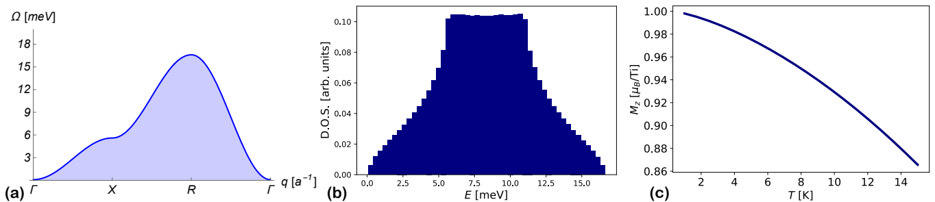
FIG. 3. (a) Linear spin-wave dispersion relation along \Gamma - X - R - \Gamma cut in Brillouin zone using idealized cubic model with J = 2.75 meV and magnon gap of \Omega_0 = 0.1 meV (after renormalizing away the Lamb shift from the orbital bath). (b) Magnon density of states (DOS) \rho(E) = \int_{\mathbf{q}} \delta(E - \Omega_{\mathbf{q}}) obtained by Monte Carlo sampling dispersion relation in (a). This is used later when we evaluate the integrals of the kinetic equation. (c) Equilibrium occupation of magnons with dispersion in (a), in terms of the magnetic moment M_z = 2\mu_B(S - n_{\text{eq}}) . We expect the Holstein-Primakoff expansion to underestimate the role of fluctuations since 1/S is not small in reality.
