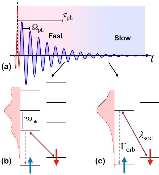
FIG. 5. (a) Time scales of pump-induced dynamics. Incident THz pulse (red) resonantly excites a phonon mode which then exhibits coherent oscillations (blue) for time scale \tau_{\text{ph}} \gg 2\pi/\Omega_{\text{ph}} . (b) These dynamics also lead to an acceleration of the spin-orbit mediated magnetization dynamics which leads to faster dynamics during the oscillations due to the appearance of a new channel for spin-flip decay via the phonon-induced sidebands. (c) After the oscillations decay, the dynamics returns to the slower time scale present in equilibrium.
