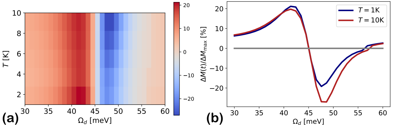
FIG. 11. (a) Plot of maximum change in magnetization as a function of initial temperature and pump frequency. (a) Color map in (\Omega_d, T) plane. We see that crossing through the resonance at \Omega_d = \Delta/2 there is a dramatic change in the sign of the effect, and that the greatest change occurs in this region. (b) Line cuts at low temperature ( T = 1 K) and high temperature ( T = 10 K). We see that the effect is slightly more efficient at increasing the magnetization when temperature is low, while it is more effective at reducing the magnetization at higher temperatures.
