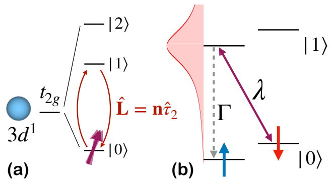
FIG. 1. (a) Splitting of Ti t_{2g} shell into non-degenerate levels by the GdFeO 3 distortion, which are then occupied by a single electron giving S = 1/2 . Interorbital coherences lead to angular momentum \mathbf{L} , which is largely quenched in equilibrium. (b) Focusing on the lowest two-levels |0\rangle and |1\rangle we find spin-flip T_1 processes in the orbital ground-state obtained from virtual orbital transitions. Spin-orbit coupling \lambda can lead to a simultaneous orbital excitation along with a spin-flip. This is then followed by a spin-independent orbital decay with rate \Gamma , shown in the level diagram. Ultimately, the decay rate is governed by the spectral overlap of the orbital bath (shown on the left schematically) with the spin-transition, which is small leading to a long-lifetime.
