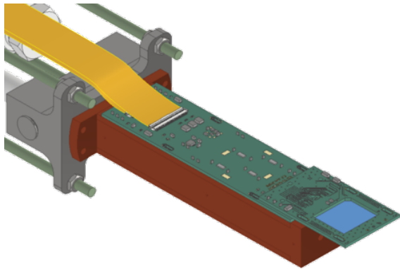
(a) 47ch planar TRISTAN detector.
