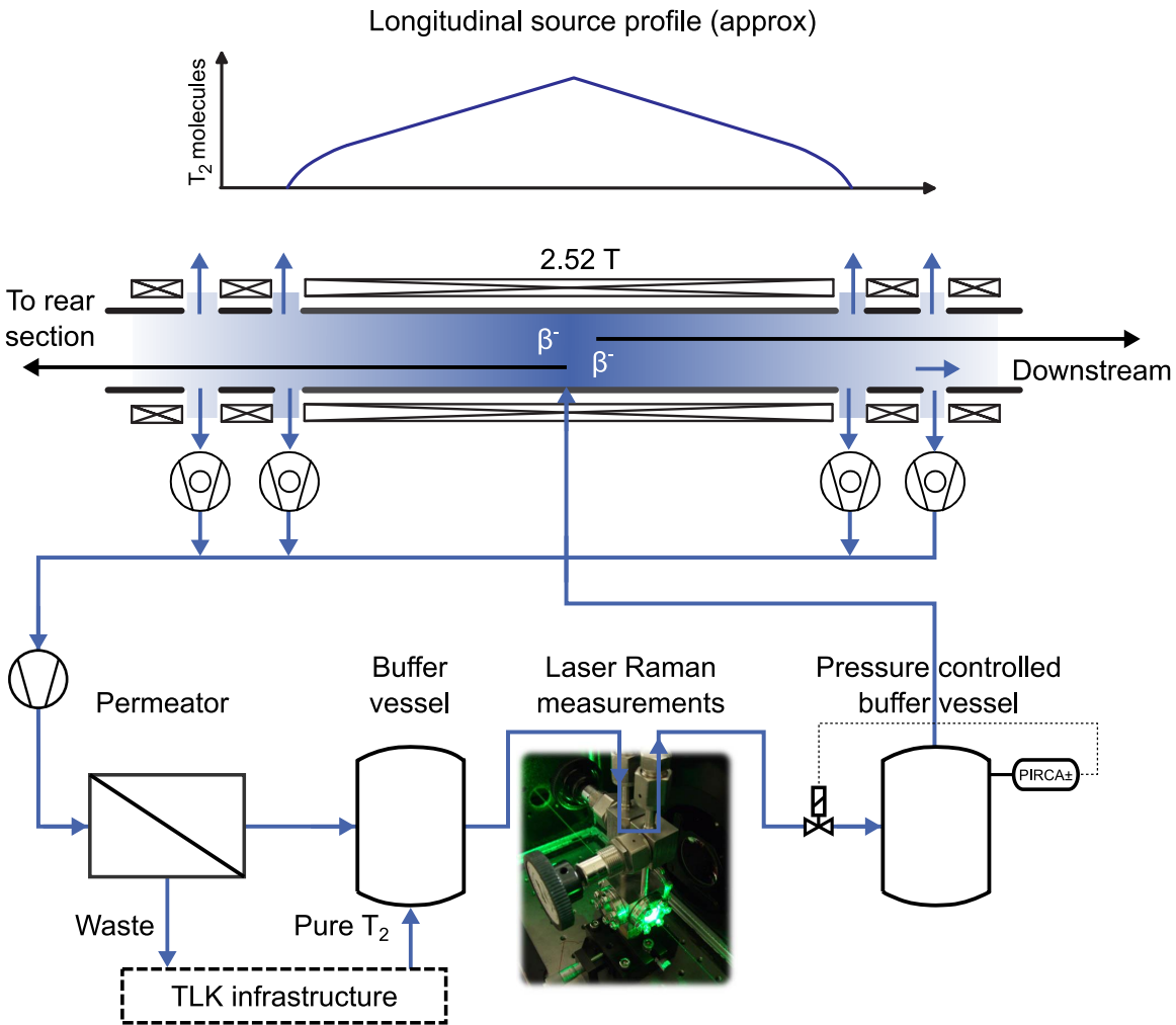
Figure 2: Simplified schematic of the windowless gaseous tritium source (WGTS) and tritium circulation loop. The temperature of the WGTS beam tube was 30\text{ K} in the first two campaigns [15, 1] and has been changed to 80\text{ K} for subsequent campaigns.
