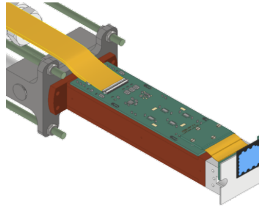
(b) 47ch 3D TRISTAN detector.
