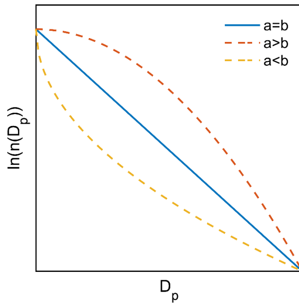
Fig. S1. Theoretical relationship between \ln(n(D_p)) and D_p under three conditions. The blue line represents the case demonstrated in the main text.
