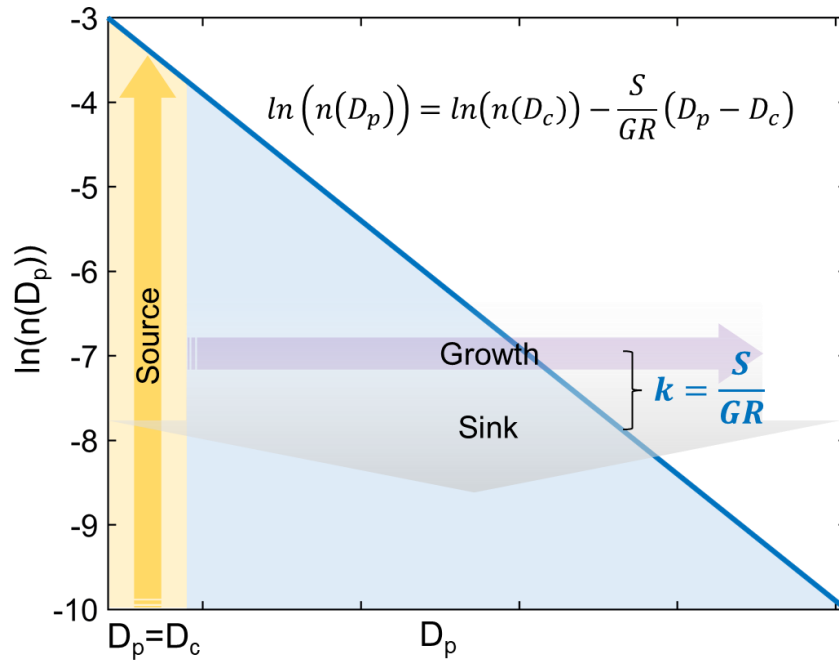
Fig. 1 Similarity of BC size distribution controlled by combined effects of growth and sink.
