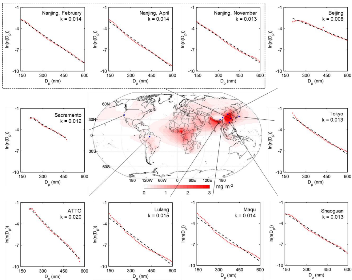
Fig. 2 Exponent distribution of BC size distributions from field measurements using single particle soot photometers (SP2) at different sites. The red dots and black lines represent the normalized size distribution of D_p and linear regression, respectively. Observations in Nanjing were conducted in different seasons. Data in Lulang and Maqu were observed over the Tibetan Plateau in spring 2021. Observations in Shaoguan, Beijing(29), Tokyo(28), Sacramento(24), and Amazon Tall Tower Observatory (ATTO) were performed in December 2020, November 2014, August 2012, June 2010, and October 2019, respectively. The map shows simulated BC radiative forcing at top of atmosphere (TOA).
