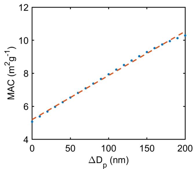
Fig. S2. Change of mass absorption cross-section (MAC) of BC with \Delta D_p . Blue dots represent the calculated MAC based on core-shell Mie theory with linear fit shown as the red line.
